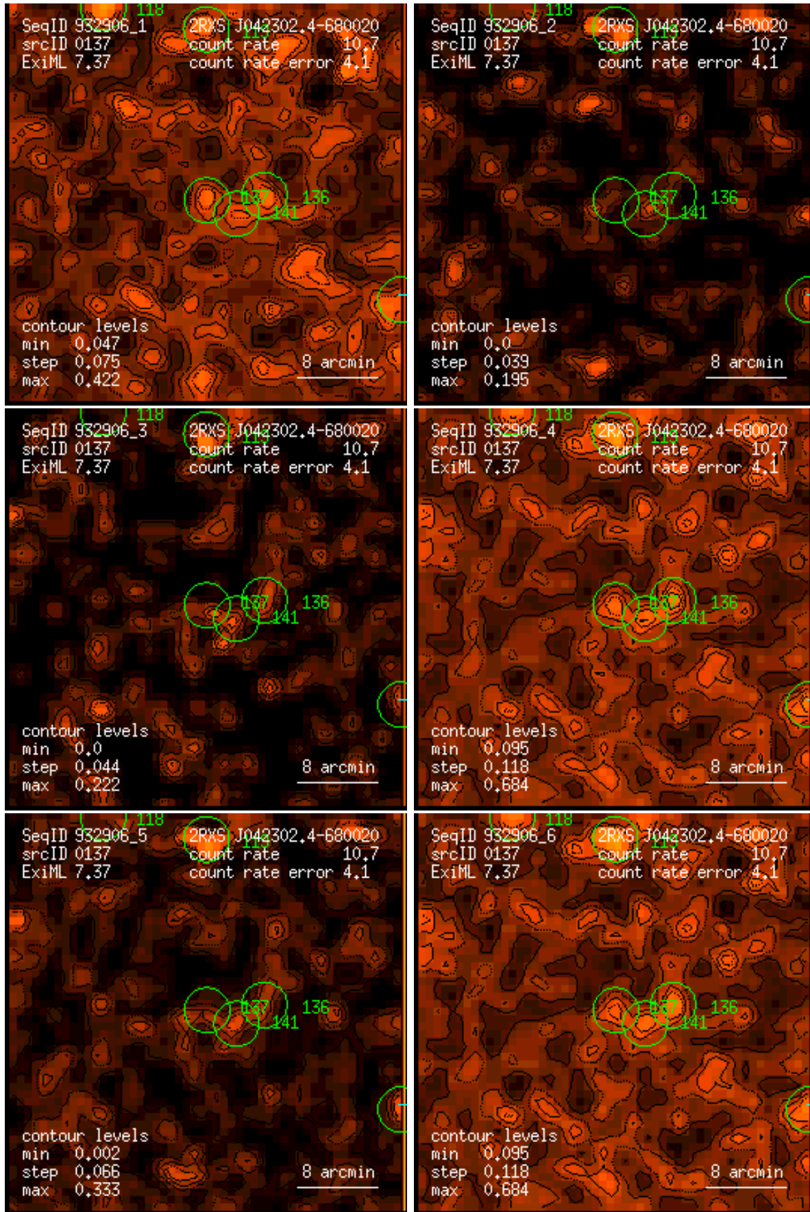
Figure 137: RASS 932906: detection 0137: band rate images, Gaussian filter: (1) PSPC channels 11 – 41, (2) 52 – 90, (3) 91 – 201, (4) 11 – 235, (5) 52 – 201, (6) 11 – 201. Broad band rates in counts/ks. Band rate contour levels in counts/ks/arcmin 2 .
