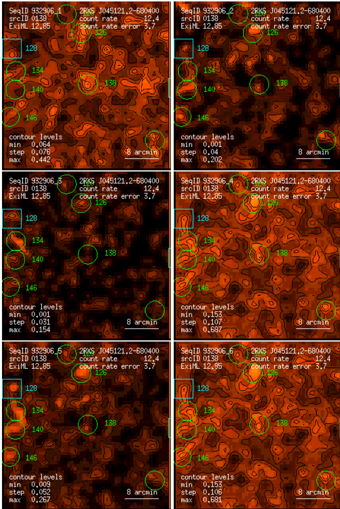
Figure 138: RASS 932906: detection 0138: band rate images, Gaussian filter: (1) PSPC channels 11 – 41, (2) 52 – 90, (3) 91 – 201, (4) 11 – 235, (5) 52 – 201, (6) 11 – 201. Broad band rates in counts/ks. Band rate contour levels in counts/ks/arcmin 2 .
