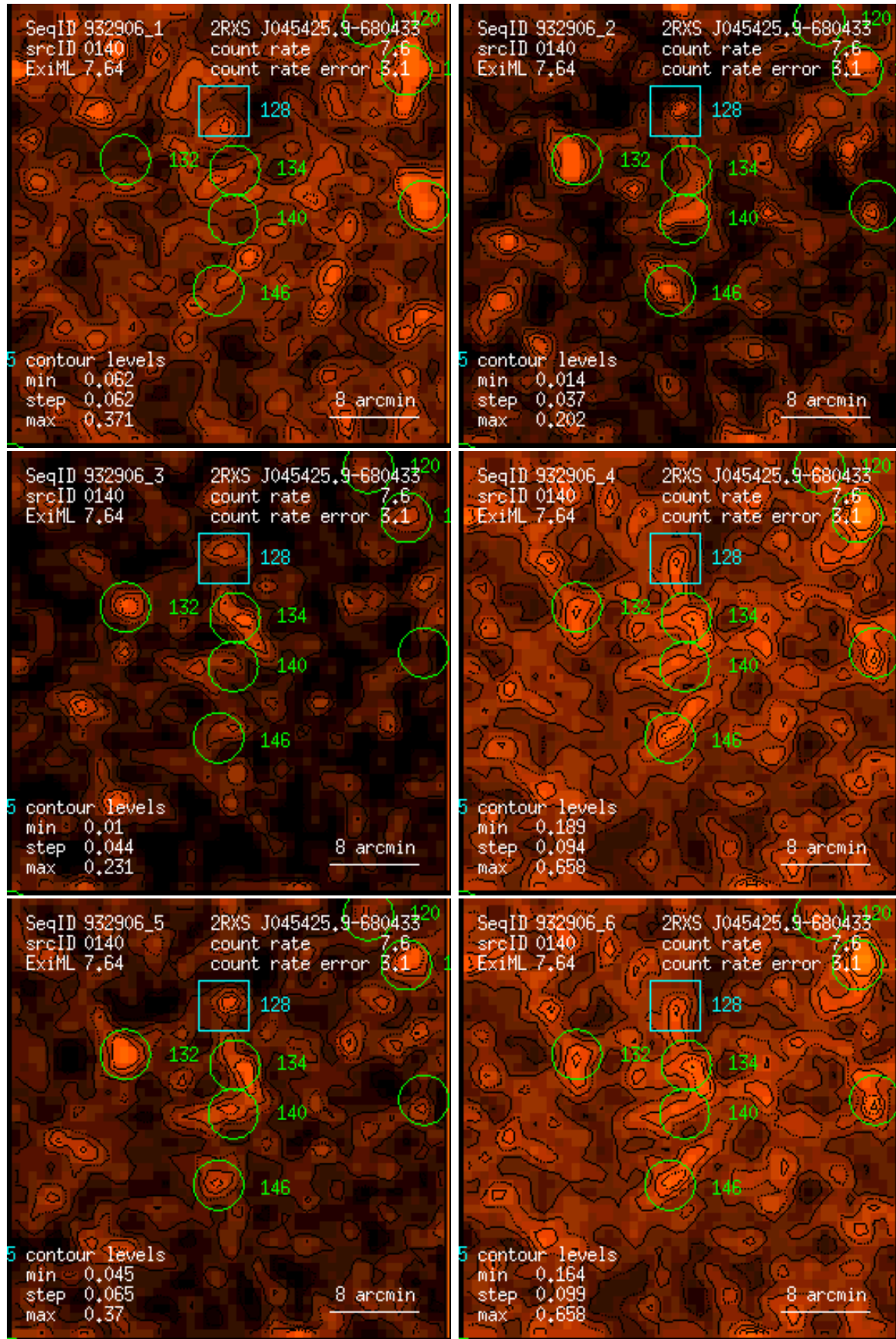
Figure 140: RASS 932906: detection 0140: band rate images, Gaussian filter: (1) PSPC channels 11 – 41, (2) 52 – 90, (3) 91 – 201, (4) 11 – 235, (5) 52 – 201, (6) 11 – 201. Broad band rates in counts/ks. Band rate contour levels in counts/ks/arcmin 2 .
