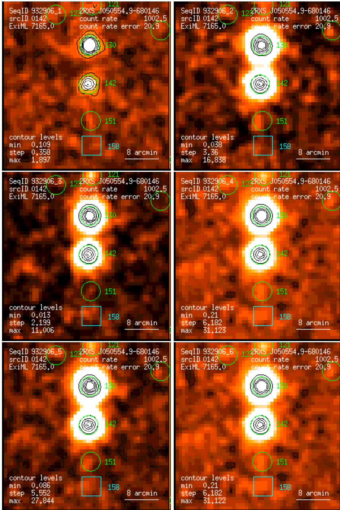
Figure 142: RASS 932906: detection 0142: band rate images, Gaussian filter: (1) PSPC channels 11 – 41, (2) 52 – 90, (3) 91 – 201, (4) 11 – 235, (5) 52 – 201, (6) 11 – 201. Broad band rates in counts/ks. Band rate contour levels in counts/ks/arcmin 2 .
