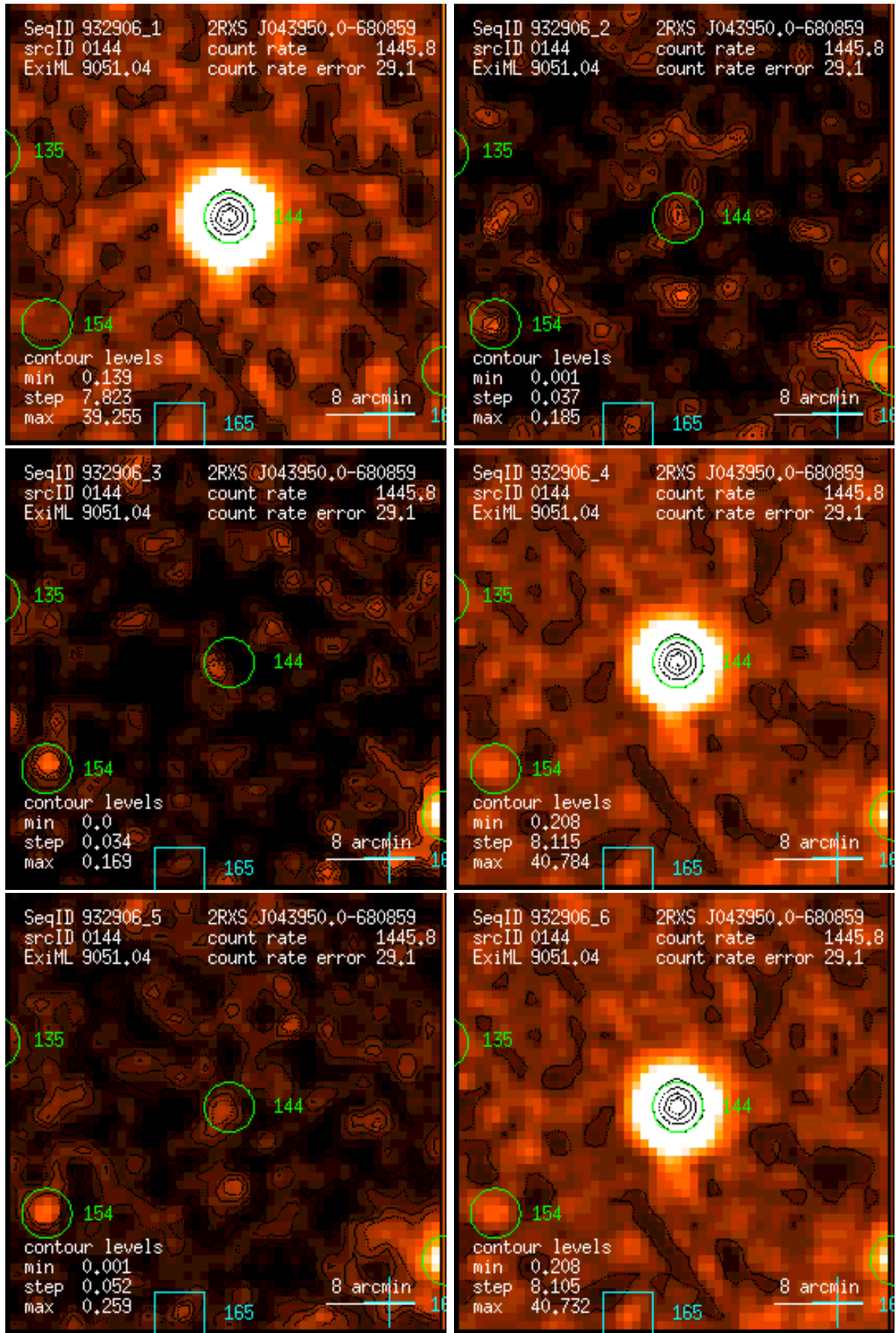
Figure 144: RASS 932906: detection 0144: band rate images, Gaussian filter: (1) PSPC channels 11 – 41, (2) 52 – 90, (3) 91 – 201, (4) 11 – 235, (5) 52 – 201, (6) 11 – 201. Broad band rates in counts/ks. Band rate contour levels in counts/ks/arcmin 2 .
