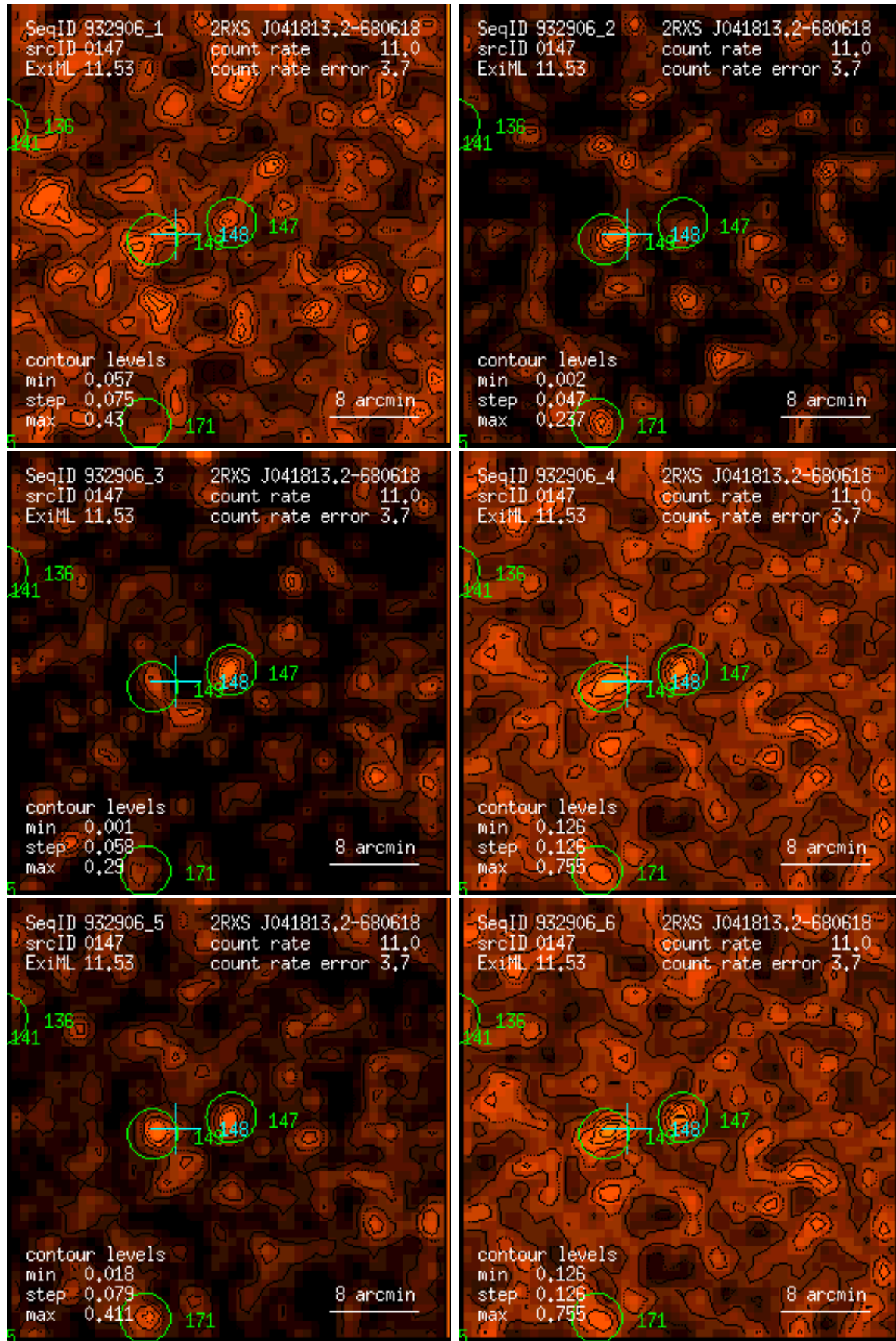
Figure 147: RASS 932906: detection 0147: band rate images, Gaussian filter: (1) PSPC channels 11 – 41, (2) 52 – 90, (3) 91 – 201, (4) 11 – 235, (5) 52 – 201, (6) 11 – 201. Broad band rates in counts/ks. Band rate contour levels in counts/ks/arcmin 2 .
