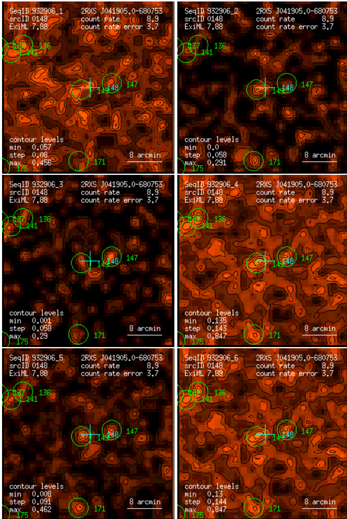
Figure 148: RASS 932906: detection 0148: band rate images, Gaussian filter: (1) PSPC channels 11 – 41, (2) 52 – 90, (3) 91 – 201, (4) 11 – 235, (5) 52 – 201, (6) 11 – 201. Broad band rates in counts/ks. Band rate contour levels in counts/ks/arcmin 2 .
