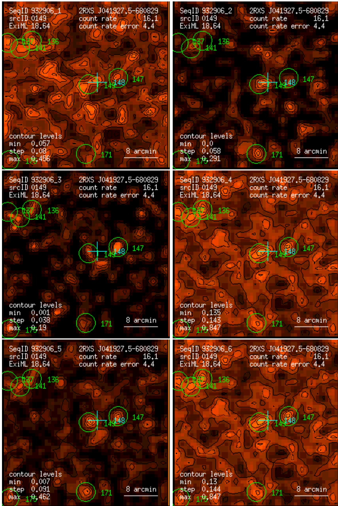
Figure 149: RASS 932906: detection 0149: band rate images, Gaussian filter: (1) PSPC channels 11 – 41, (2) 52 – 90, (3) 91 – 201, (4) 11 – 235, (5) 52 – 201, (6) 11 – 201. Broad band rates in counts/ks. Band rate contour levels in counts/ks/arcmin 2 .
