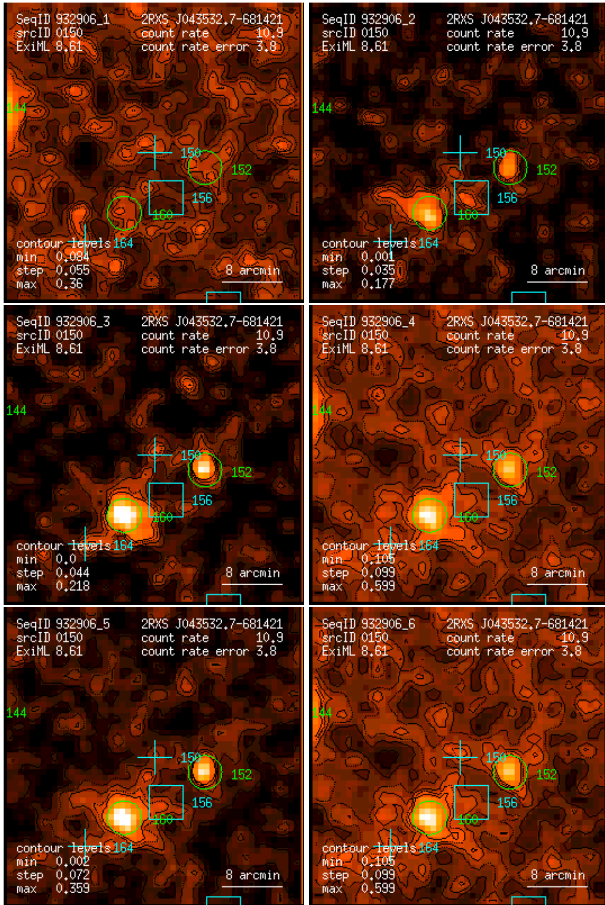
Figure 150: RASS 932906: detection 0150: band rate images, Gaussian filter: (1) PSPC channels 11 – 41, (2) 52 – 90, (3) 91 – 201, (4) 11 – 235, (5) 52 – 201, (6) 11 – 201. Broad band rates in counts/ks. Band rate contour levels in counts/ks/arcmin 2 .
