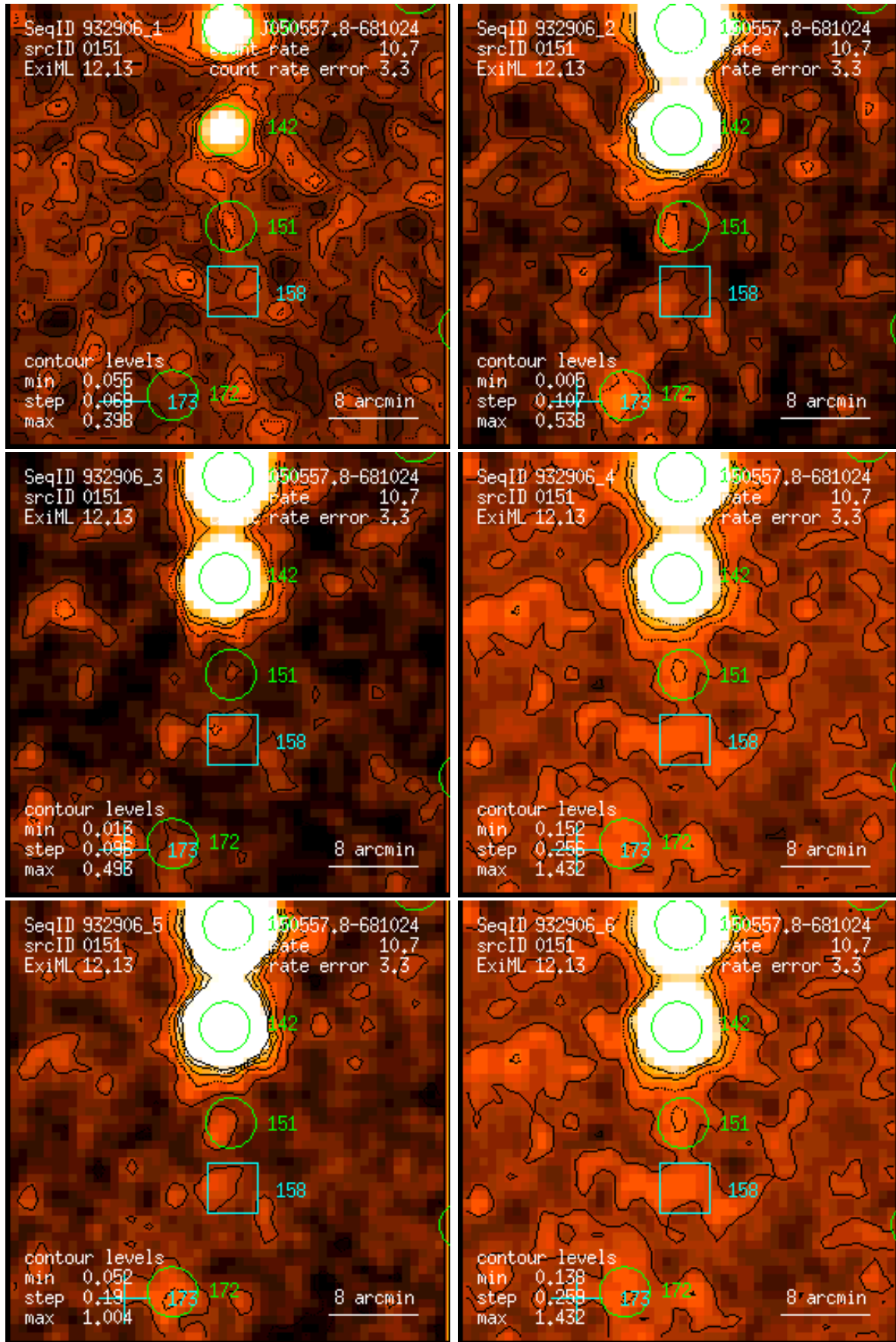
Figure 151: RASS 932906: detection 0151: band rate images, Gaussian filter: (1) PSPC channels 11 – 41, (2) 52 – 90, (3) 91 – 201, (4) 11 – 235, (5) 52 – 201, (6) 11 – 201. Broad band rates in counts/ks. Band rate contour levels in counts/ks/arcmin 2 .
