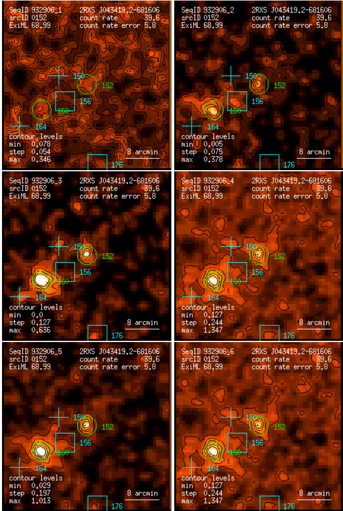
Figure 152: RASS 932906: detection 0152: band rate images, Gaussian filter: (1) PSPC channels 11 – 41, (2) 52 – 90, (3) 91 – 201, (4) 11 – 235, (5) 52 – 201, (6) 11 – 201. Broad band rates in counts/ks. Band rate contour levels in counts/ks/arcmin 2 .
