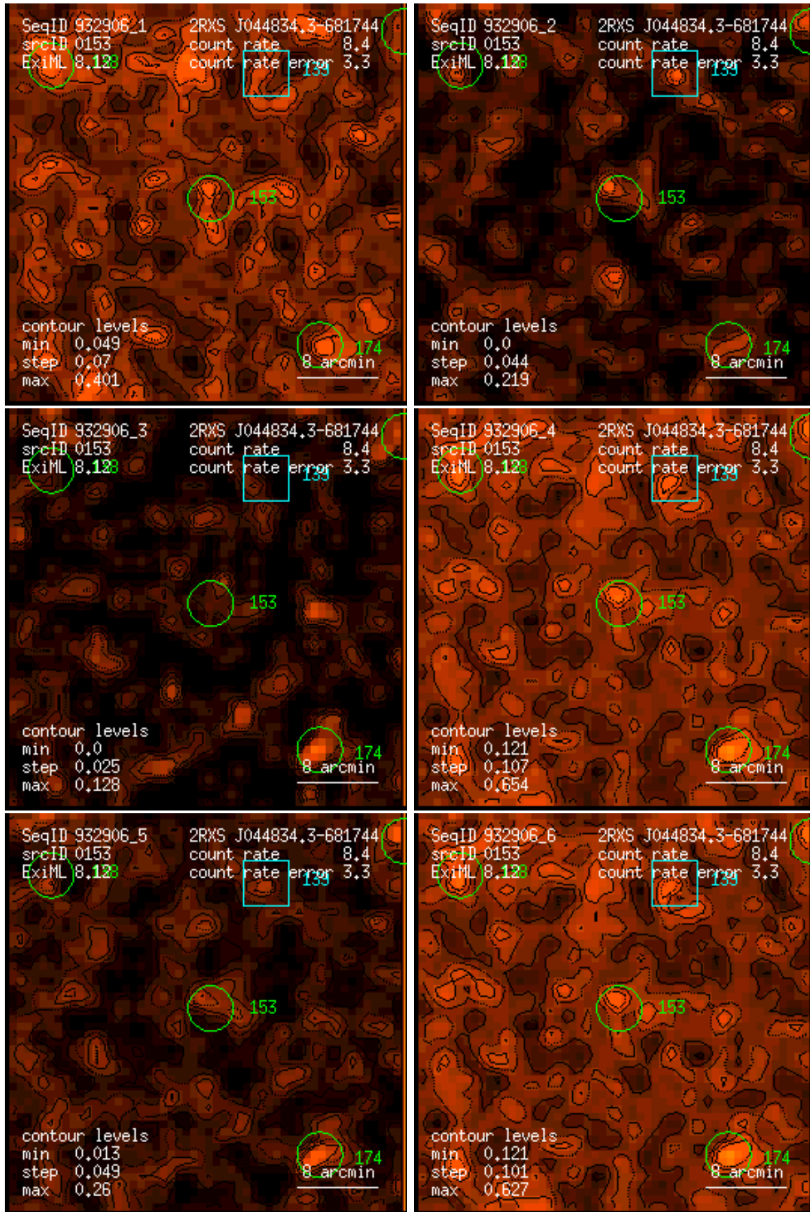
Figure 153: RASS 932906: detection 0153: band rate images, Gaussian filter: (1) PSPC channels 11 – 41, (2) 52 – 90, (3) 91 – 201, (4) 11 – 235, (5) 52 – 201, (6) 11 – 201. Broad band rates in counts/ks. Band rate contour levels in counts/ks/arcmin 2 .
