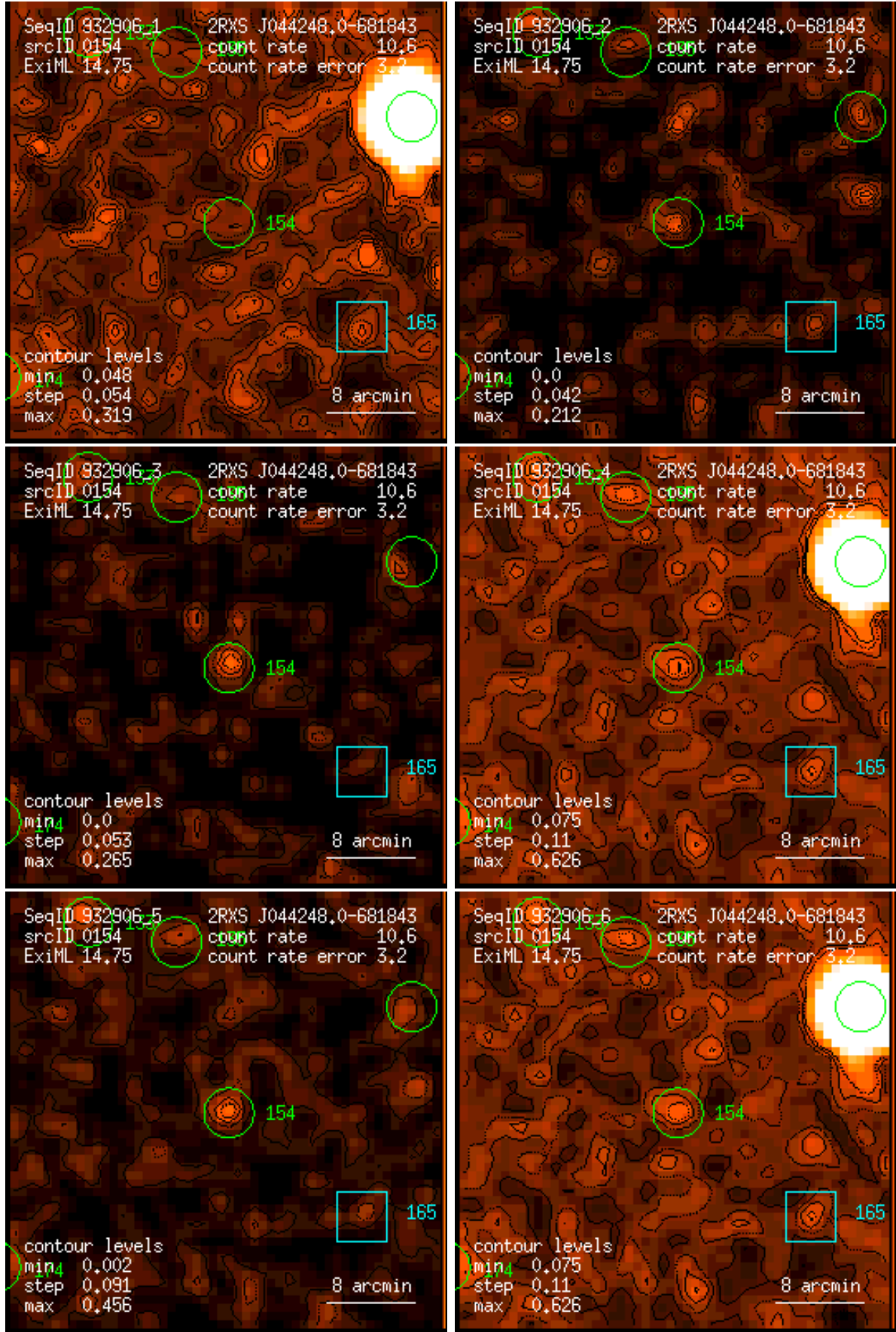
Figure 154: RASS 932906: detection 0154: band rate images, Gaussian filter: (1) PSPC channels 11 – 41, (2) 52 – 90, (3) 91 – 201, (4) 11 – 235, (5) 52 – 201, (6) 11 – 201. Broad band rates in counts/ks. Band rate contour levels in counts/ks/arcmin 2 .
