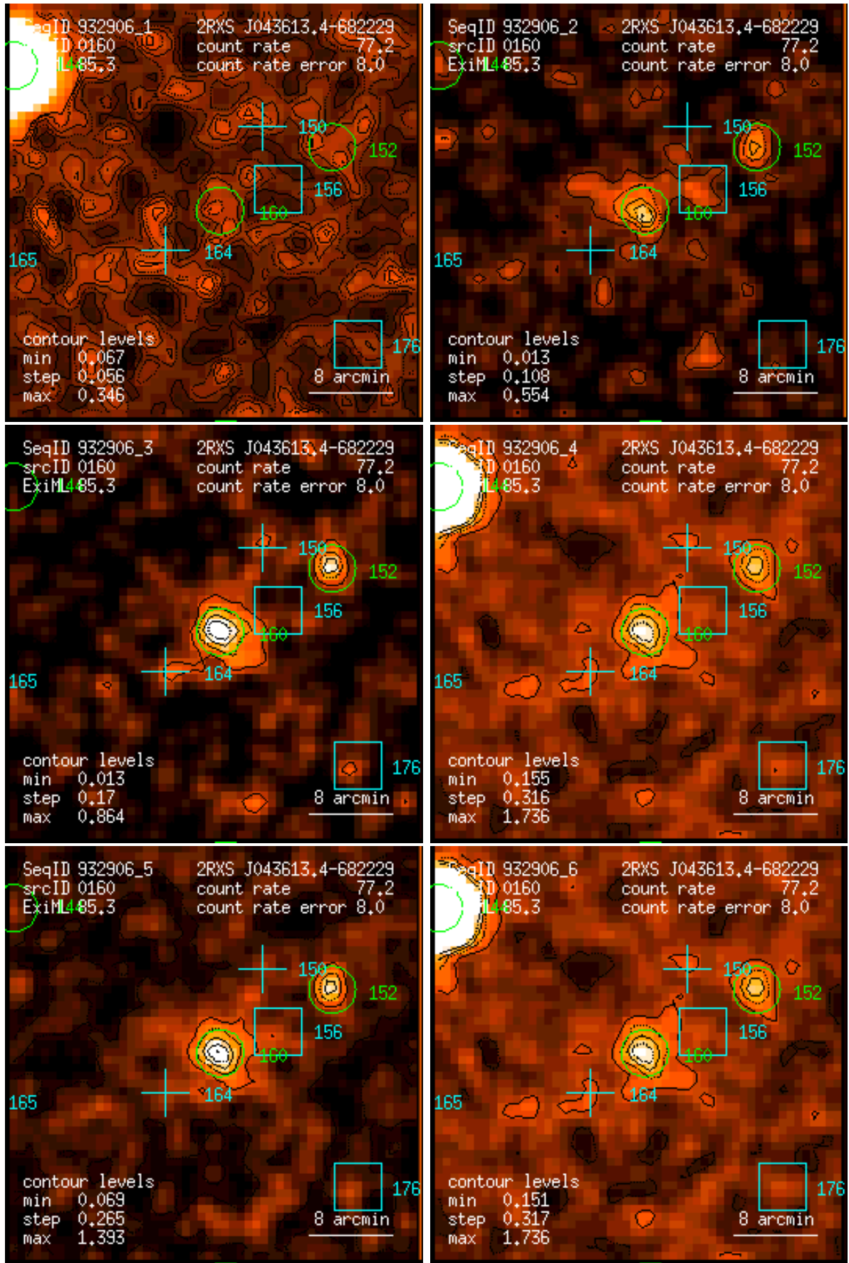
Figure 160: RASS 932906: detection 0160: band rate images, Gaussian filter: (1) PSPC channels 11 – 41, (2) 52 – 90, (3) 91 – 201, (4) 11 – 235, (5) 52 – 201, (6) 11 – 201. Broad band rates in counts/ks. Band rate contour levels in counts/ks/arcmin 2 .
