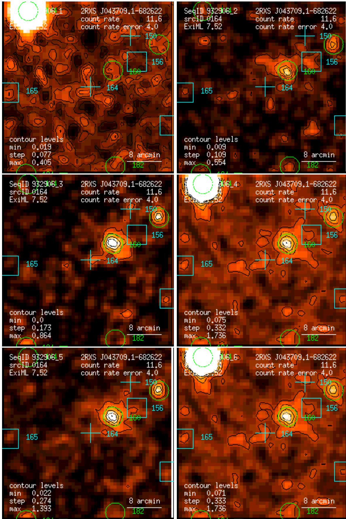
Figure 164: RASS 932906: detection 0164: band rate images, Gaussian filter: (1) PSPC channels 11 – 41, (2) 52 – 90, (3) 91 – 201, (4) 11 – 235, (5) 52 – 201, (6) 11 – 201. Broad band rates in counts/ks. Band rate contour levels in counts/ks/arcmin 2 .
