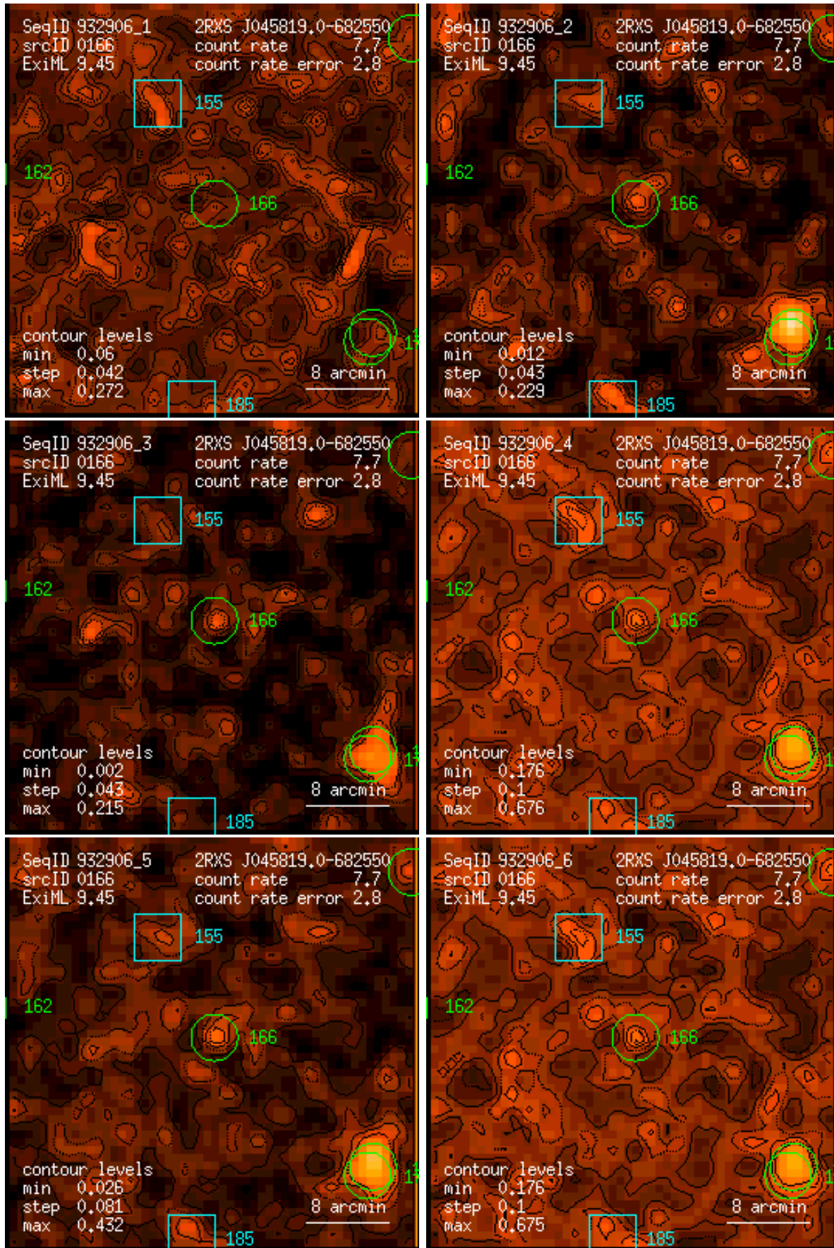
Figure 166: RASS 932906: detection 0166: band rate images, Gaussian filter: (1) PSPC channels 11 – 41, (2) 52 – 90, (3) 91 – 201, (4) 11 – 235, (5) 52 – 201, (6) 11 – 201. Broad band rates in counts/ks. Band rate contour levels in counts/ks/arcmin 2 .
