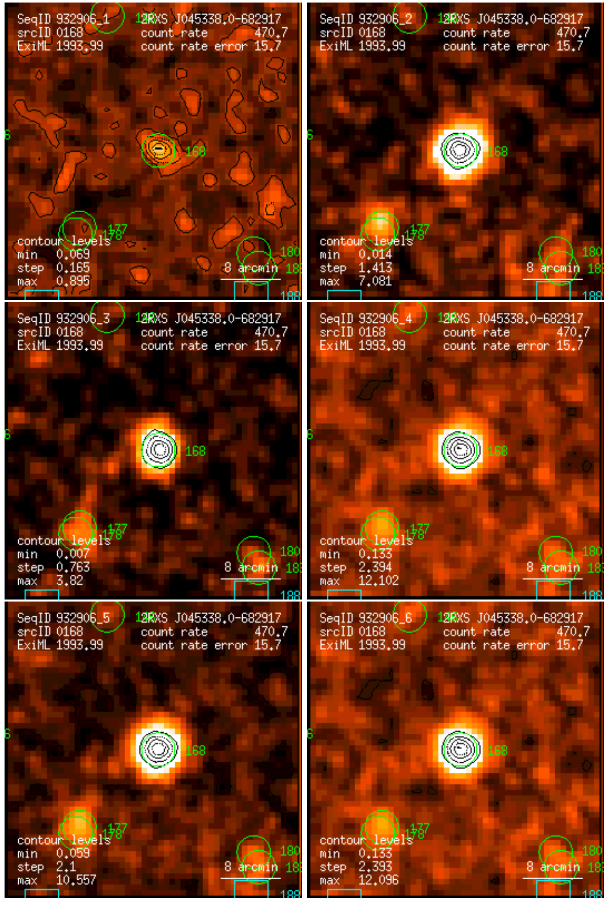
Figure 168: RASS 932906: detection 0168: band rate images, Gaussian filter: (1) PSPC channels 11 – 41, (2) 52 – 90, (3) 91 – 201, (4) 11 – 235, (5) 52 – 201, (6) 11 – 201. Broad band rates in counts/ks. Band rate contour levels in counts/ks/arcmin 2 .
