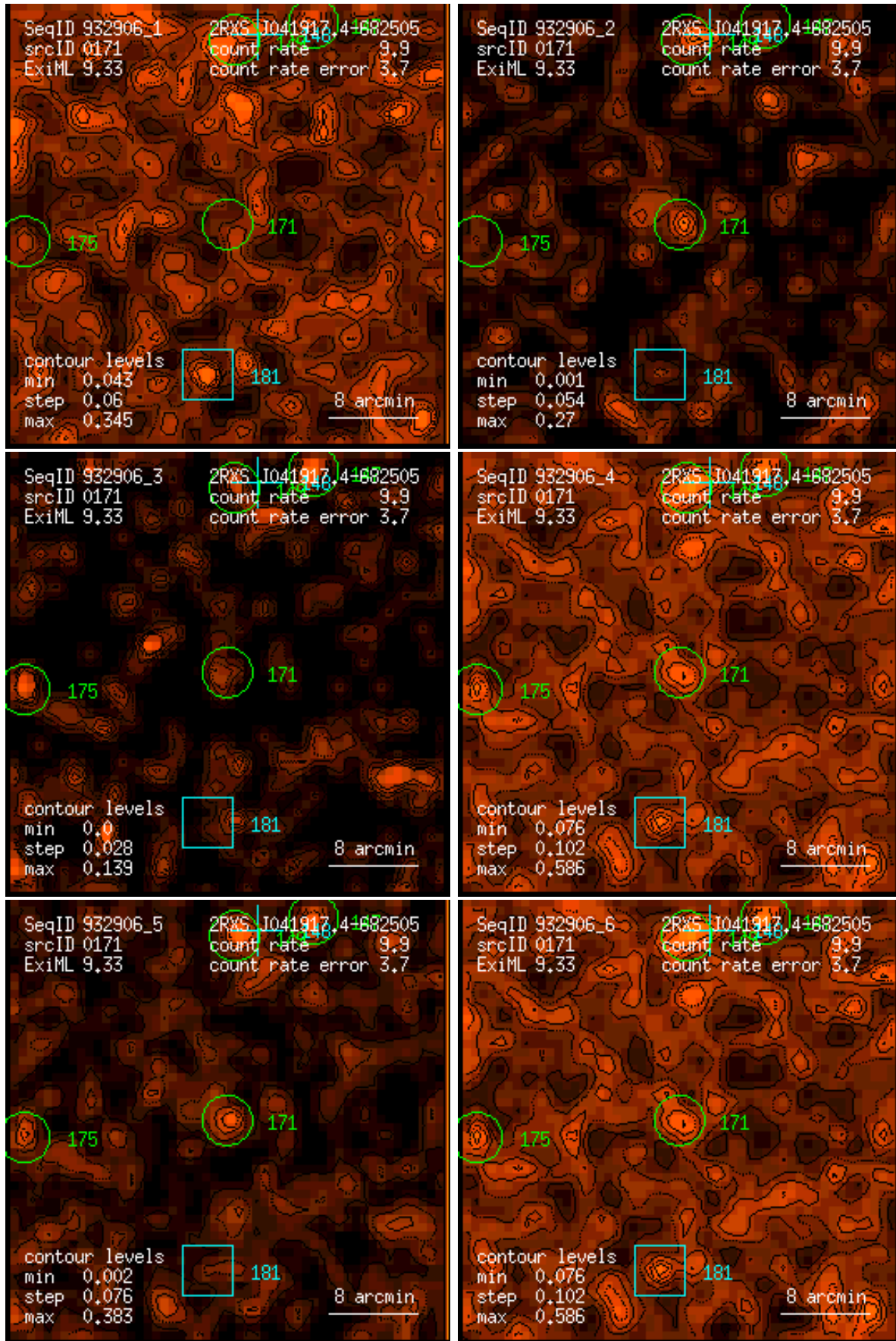
Figure 171: RASS 932906: detection 0171: band rate images, Gaussian filter: (1) PSPC channels 11 – 41, (2) 52 – 90, (3) 91 – 201, (4) 11 – 235, (5) 52 – 201, (6) 11 – 201. Broad band rates in counts/ks. Band rate contour levels in counts/ks/arcmin 2 .
