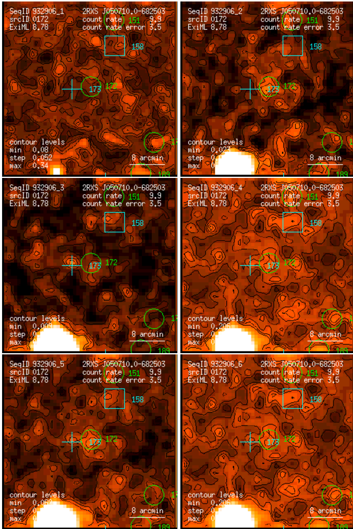
Figure 172: RASS 932906: detection 0172: band rate images, Gaussian filter: (1) PSPC channels 11 – 41, (2) 52 – 90, (3) 91 – 201, (4) 11 – 235, (5) 52 – 201, (6) 11 – 201. Broad band rates in counts/ks. Band rate contour levels in counts/ks/arcmin 2 .
