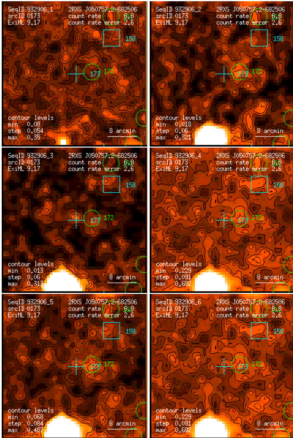
Figure 173: RASS 932906: detection 0173: band rate images, Gaussian filter: (1) PSPC channels 11 – 41, (2) 52 – 90, (3) 91 – 201, (4) 11 – 235, (5) 52 – 201, (6) 11 – 201. Broad band rates in counts/ks. Band rate contour levels in counts/ks/arcmin 2 .
