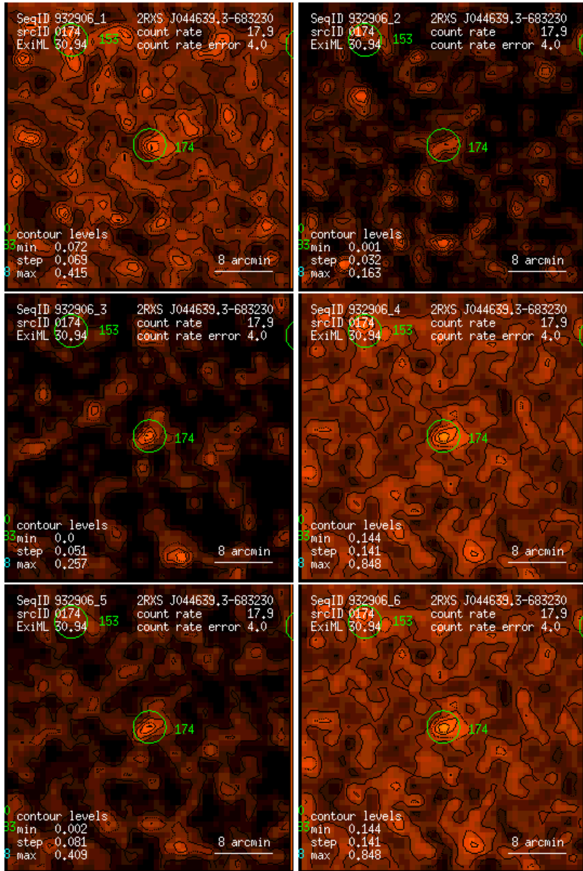
Figure 174: RASS 932906: detection 0174: band rate images, Gaussian filter: (1) PSPC channels 11 – 41, (2) 52 – 90, (3) 91 – 201, (4) 11 – 235, (5) 52 – 201, (6) 11 – 201. Broad band rates in counts/ks. Band rate contour levels in counts/ks/arcmin 2 .
