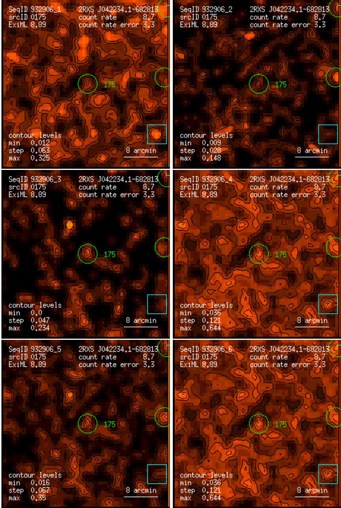
Figure 175: RASS 932906: detection 0175: band rate images, Gaussian filter: (1) PSPC channels 11 – 41, (2) 52 – 90, (3) 91 – 201, (4) 11 – 235, (5) 52 – 201, (6) 11 – 201. Broad band rates in counts/ks. Band rate contour levels in counts/ks/arcmin 2 .
