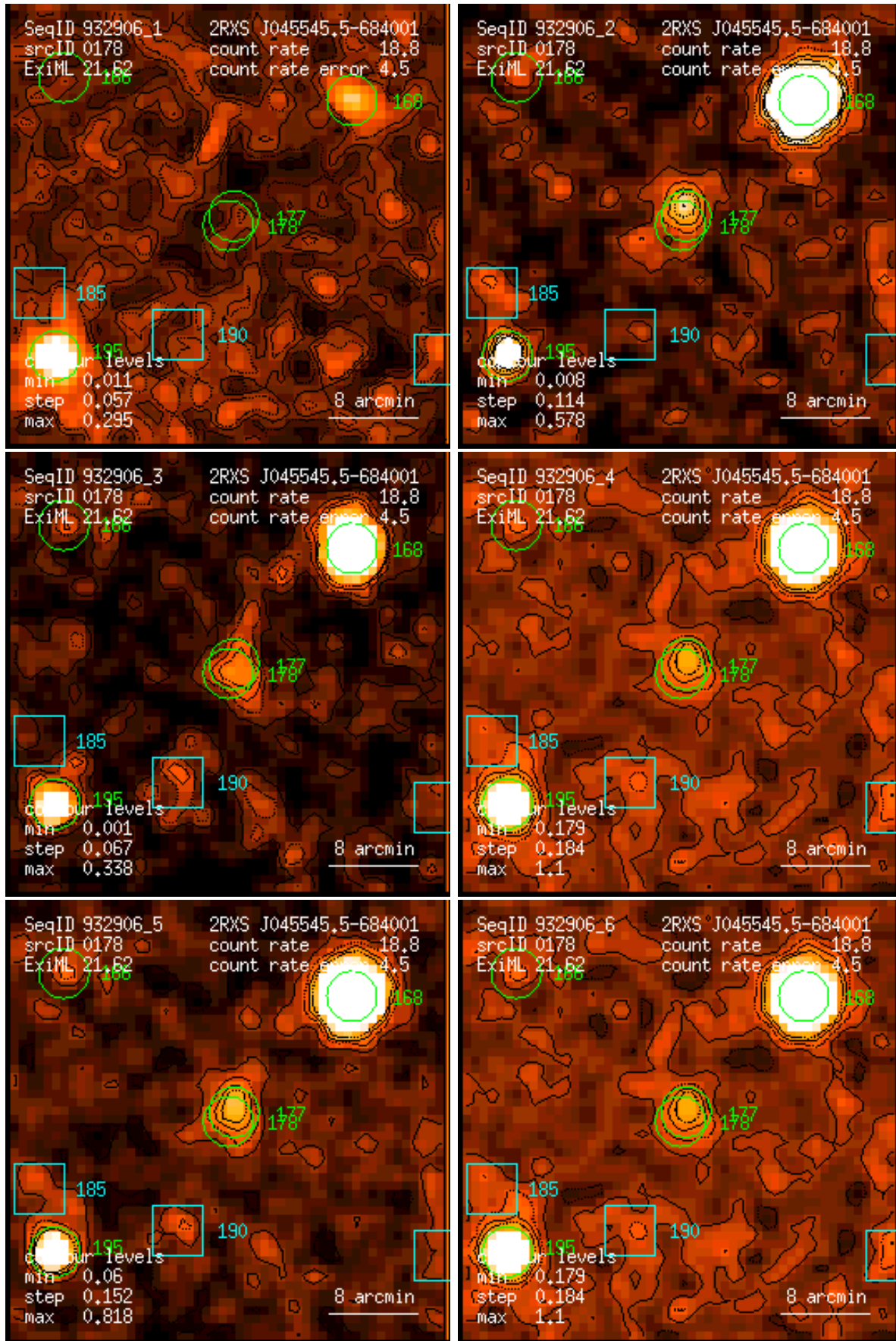
Figure 178: RASS 932906: detection 0178: band rate images, Gaussian filter: (1) PSPC channels 11 – 41, (2) 52 – 90, (3) 91 – 201, (4) 11 – 235, (5) 52 – 201, (6) 11 – 201. Broad band rates in counts/ks. Band rate contour levels in counts/ks/arcmin 2 .
