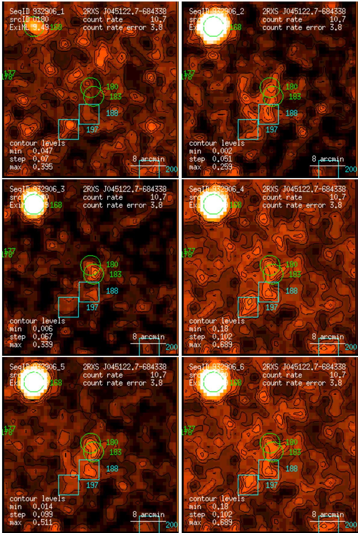
Figure 180: RASS 932906: detection 0180: band rate images, Gaussian filter: (1) PSPC channels 11 – 41, (2) 52 – 90, (3) 91 – 201, (4) 11 – 235, (5) 52 – 201, (6) 11 – 201. Broad band rates in counts/ks. Band rate contour levels in counts/ks/arcmin 2 .
