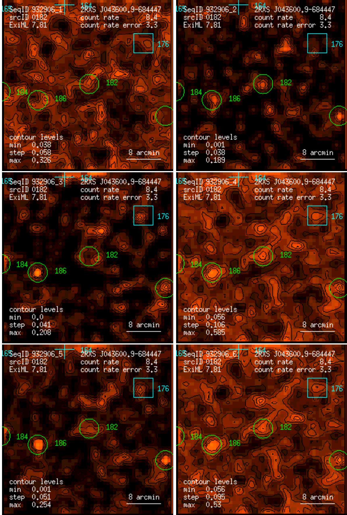
Figure 182: RASS 932906: detection 0182: band rate images, Gaussian filter: (1) PSPC channels 11 – 41, (2) 52 – 90, (3) 91 – 201, (4) 11 – 235, (5) 52 – 201, (6) 11 – 201. Broad band rates in counts/ks. Band rate contour levels in counts/ks/arcmin 2 .
