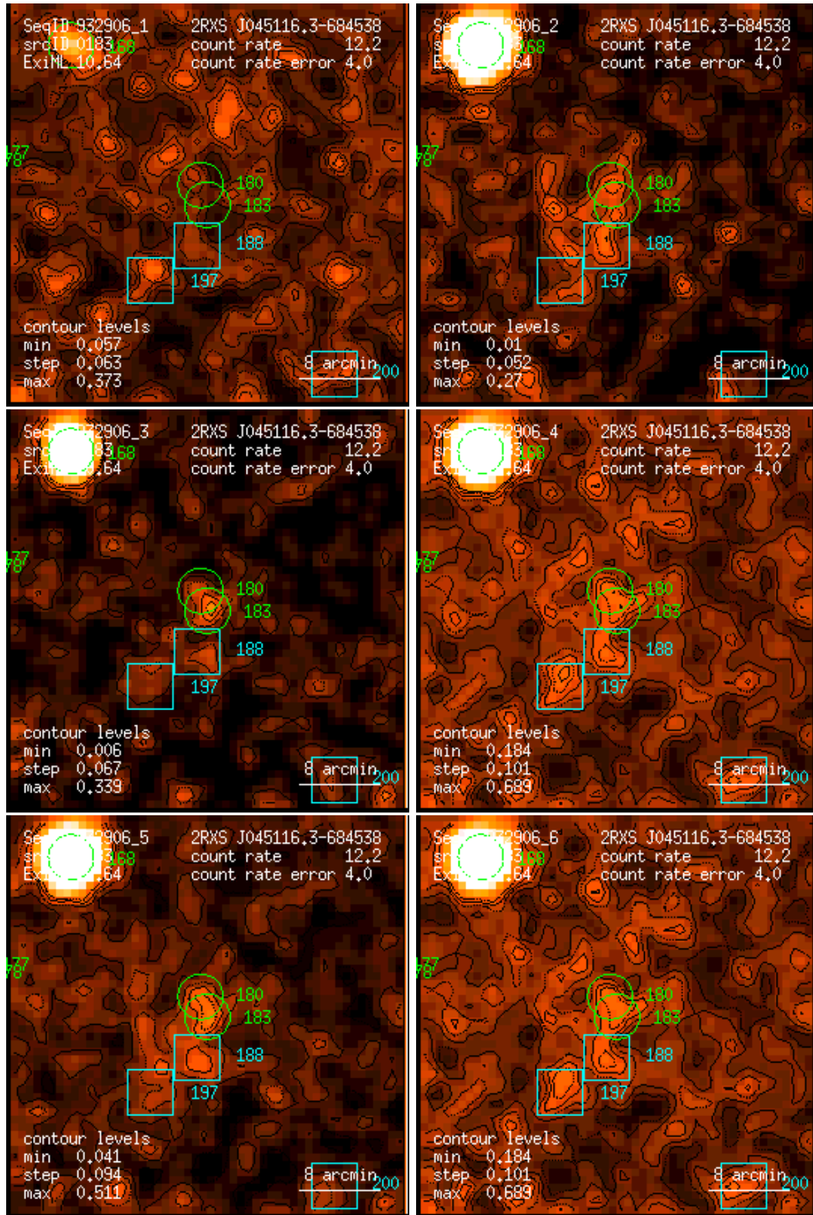
Figure 183: RASS 932906: detection 0183: band rate images, Gaussian filter: (1) PSPC channels 11 – 41, (2) 52 – 90, (3) 91 – 201, (4) 11 – 235, (5) 52 – 201, (6) 11 – 201. Broad band rates in counts/ks. Band rate contour levels in counts/ks/arcmin 2 .
