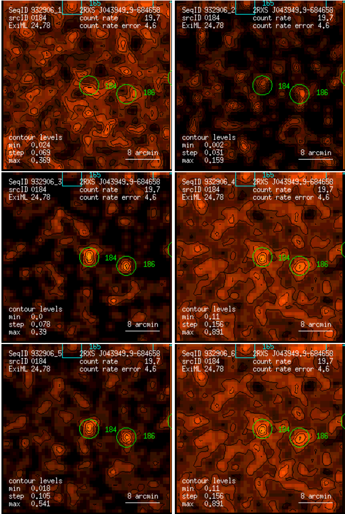
Figure 184: RASS 932906: detection 0184: band rate images, Gaussian filter: (1) PSPC channels 11 – 41, (2) 52 – 90, (3) 91 – 201, (4) 11 – 235, (5) 52 – 201, (6) 11 – 201. Broad band rates in counts/ks. Band rate contour levels in counts/ks/arcmin 2 .
