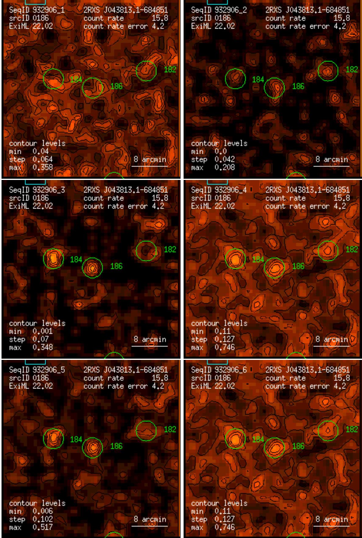
Figure 186: RASS 932906: detection 0186: band rate images, Gaussian filter: (1) PSPC channels 11 – 41, (2) 52 – 90, (3) 91 – 201, (4) 11 – 235, (5) 52 – 201, (6) 11 – 201. Broad band rates in counts/ks. Band rate contour levels in counts/ks/arcmin 2 .
