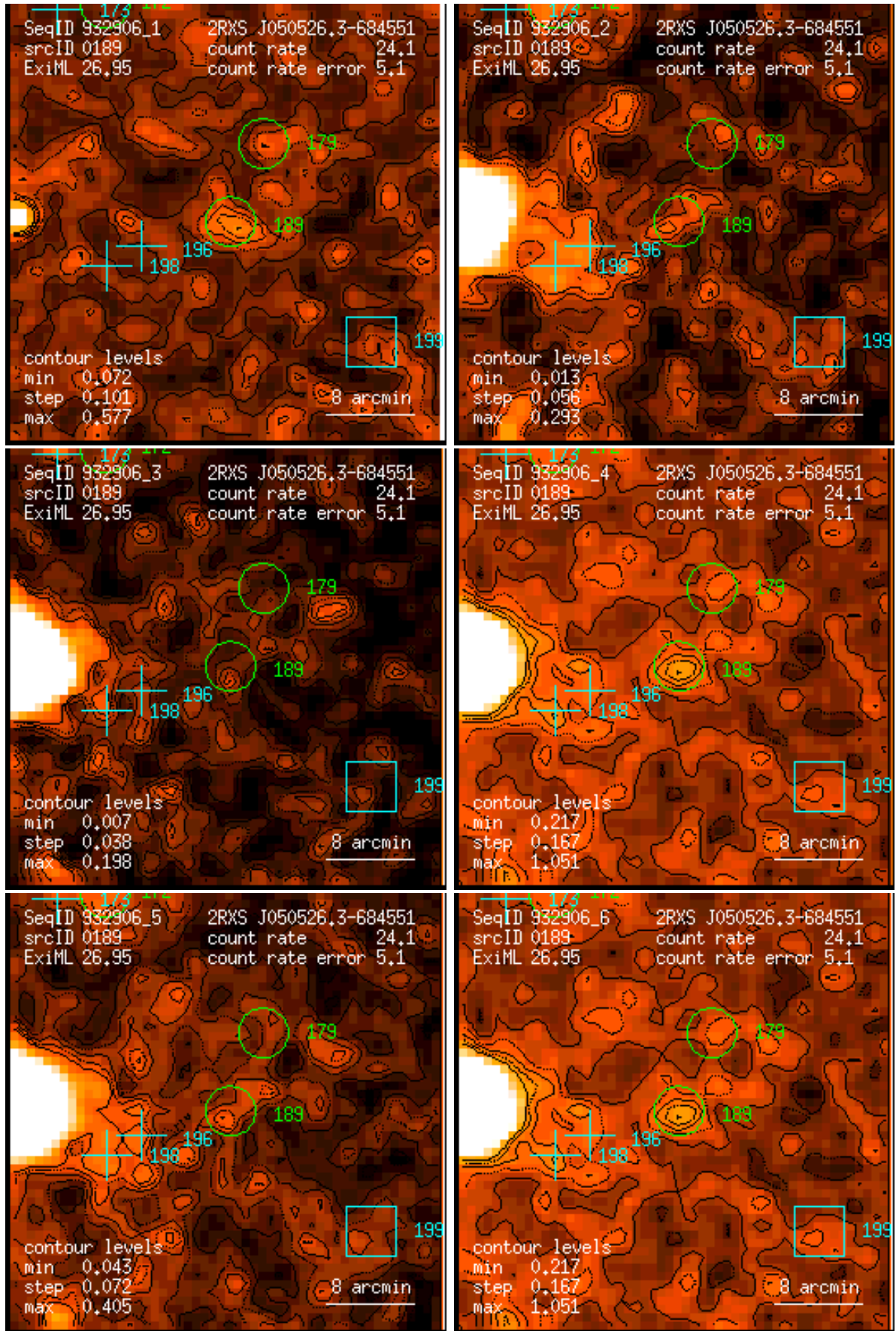
Figure 189: RASS 932906: detection 0189: band rate images, Gaussian filter: (1) PSPC channels 11 – 41, (2) 52 – 90, (3) 91 – 201, (4) 11 – 235, (5) 52 – 201, (6) 11 – 201. Broad band rates in counts/ks. Band rate contour levels in counts/ks/arcmin 2 .
