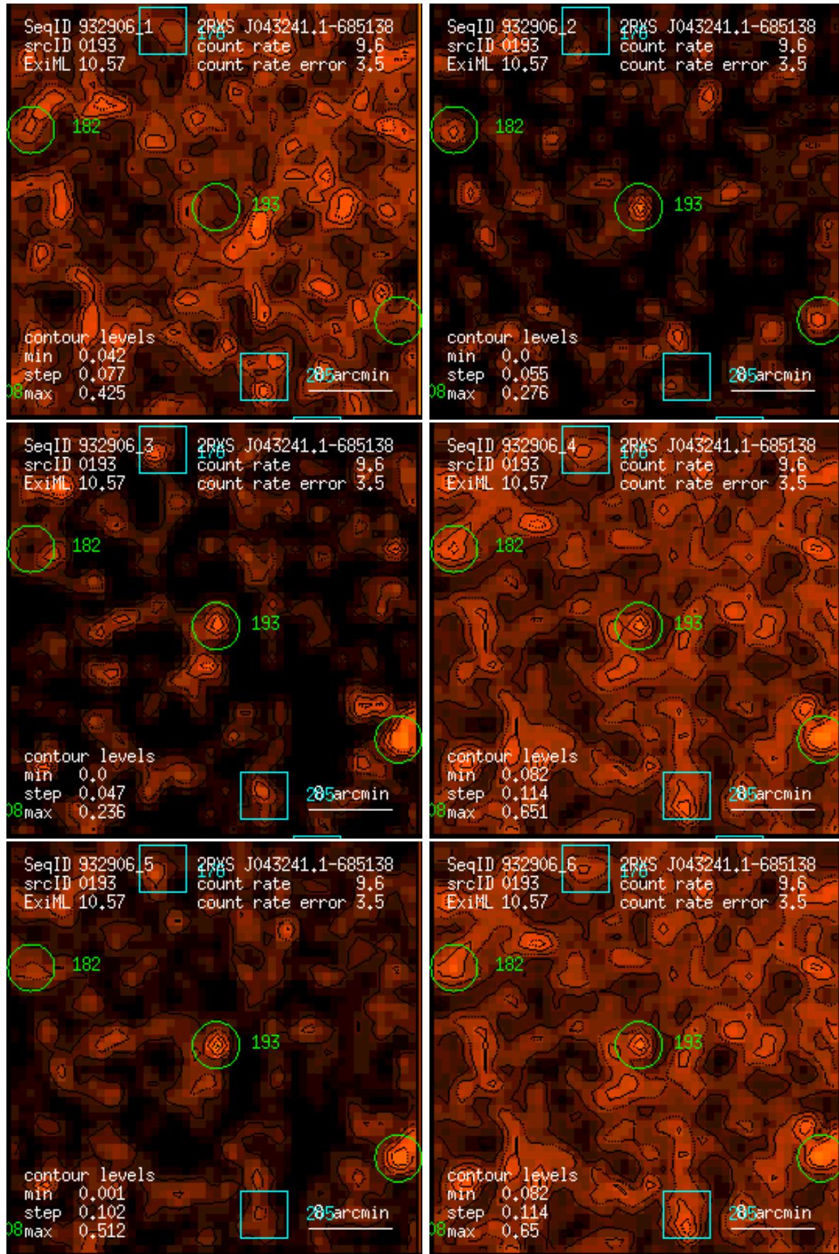
Figure 193: RASS 932906: detection 0193: band rate images, Gaussian filter: (1) PSPC channels 11 – 41, (2) 52 – 90, (3) 91 – 201, (4) 11 – 235, (5) 52 – 201, (6) 11 – 201. Broad band rates in counts/ks. Band rate contour levels in counts/ks/arcmin 2 .
