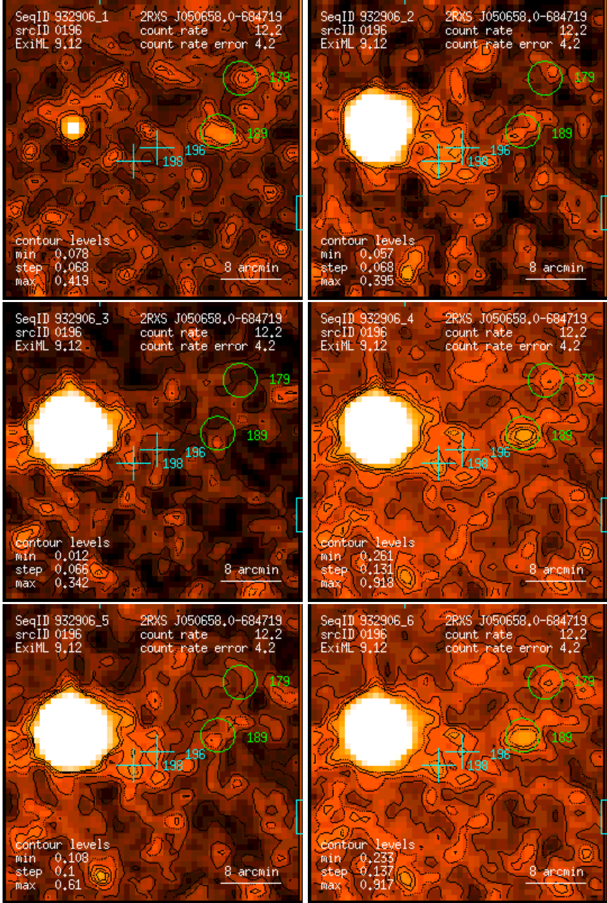
Figure 196: RASS 932906: detection 0196: band rate images, Gaussian filter: (1) PSPC channels 11 – 41, (2) 52 – 90, (3) 91 – 201, (4) 11 – 235, (5) 52 – 201, (6) 11 – 201. Broad band rates in counts/ks. Band rate contour levels in counts/ks/arcmin 2 .
