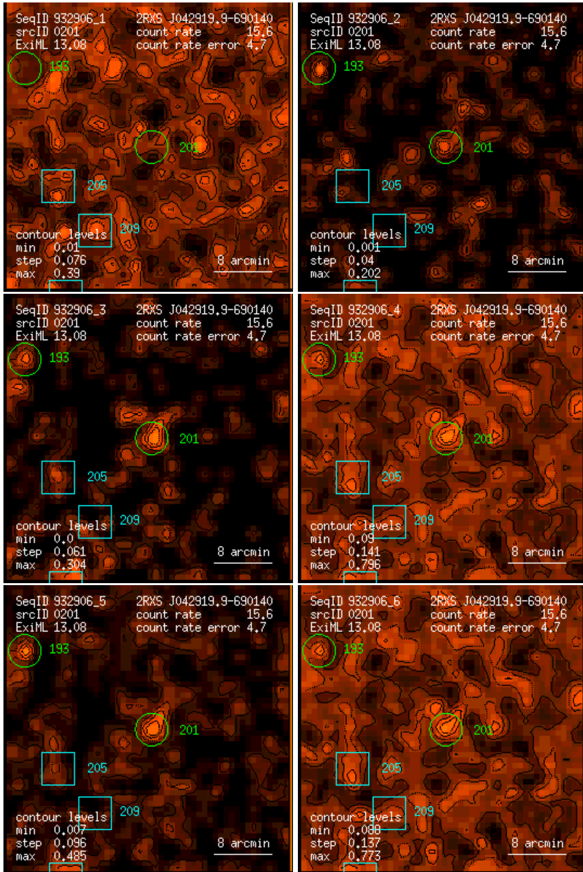
Figure 201: RASS 932906: detection 0201: band rate images, Gaussian filter: (1) PSPC channels 11 – 41, (2) 52 – 90, (3) 91 – 201, (4) 11 – 235, (5) 52 – 201, (6) 11 – 201. Broad band rates in counts/ks. Band rate contour levels in counts/ks/arcmin 2 .
