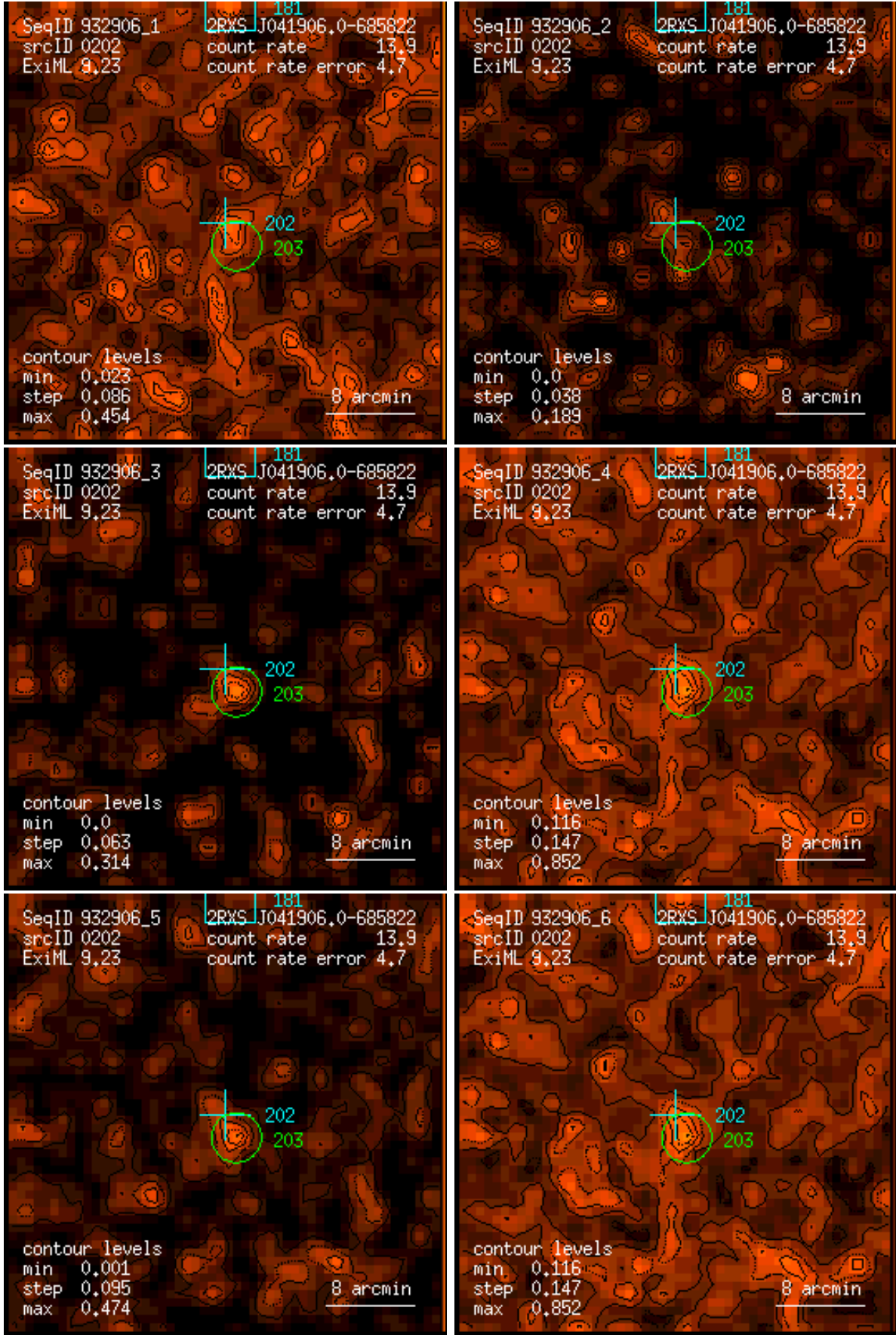
Figure 202: RASS 932906: detection 0202: band rate images, Gaussian filter: (1) PSPC channels 11 – 41, (2) 52 – 90, (3) 91 – 201, (4) 11 – 235, (5) 52 – 201, (6) 11 – 201. Broad band rates in counts/ks. Band rate contour levels in counts/ks/arcmin 2 .
