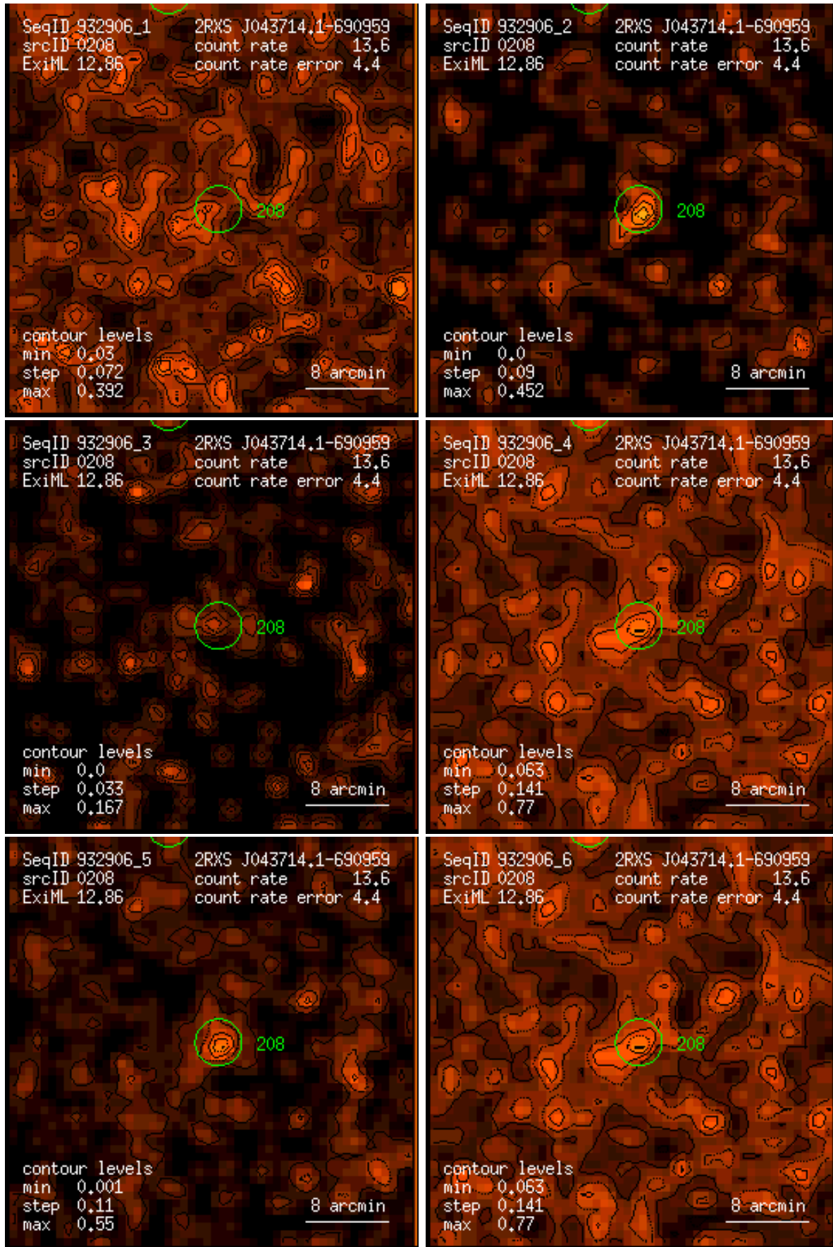
Figure 208: RASS 932906: detection 0208: band rate images, Gaussian filter: (1) PSPC channels 11 – 41, (2) 52 – 90, (3) 91 – 201, (4) 11 – 235, (5) 52 – 201, (6) 11 – 201. Broad band rates in counts/ks. Band rate contour levels in counts/ks/arcmin 2 .
