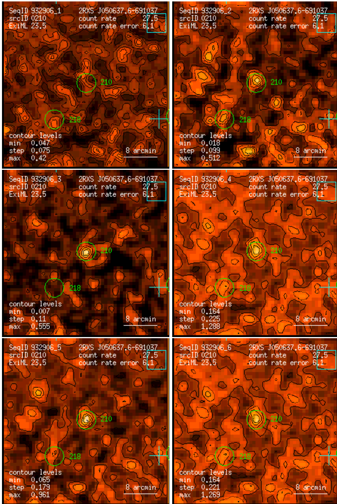
Figure 210: RASS 932906: detection 0210: band rate images, Gaussian filter: (1) PSPC channels 11 – 41, (2) 52 – 90, (3) 91 – 201, (4) 11 – 235, (5) 52 – 201, (6) 11 – 201. Broad band rates in counts/ks. Band rate contour levels in counts/ks/arcmin 2 .
