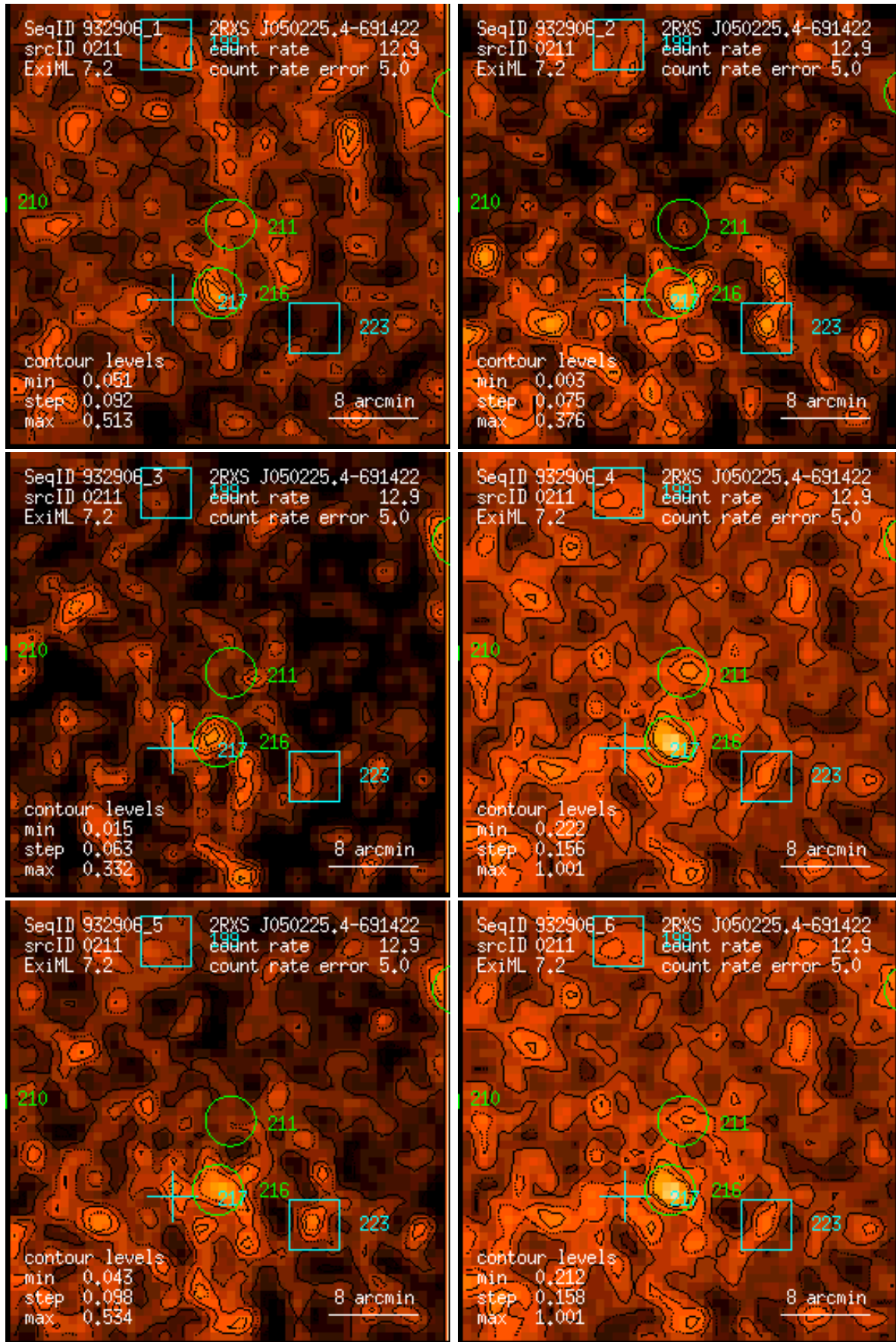
Figure 211: RASS 932906: detection 0211: band rate images, Gaussian filter: (1) PSPC channels 11 – 41, (2) 52 – 90, (3) 91 – 201, (4) 11 – 235, (5) 52 – 201, (6) 11 – 201. Broad band rates in counts/ks. Band rate contour levels in counts/ks/arcmin 2 .
