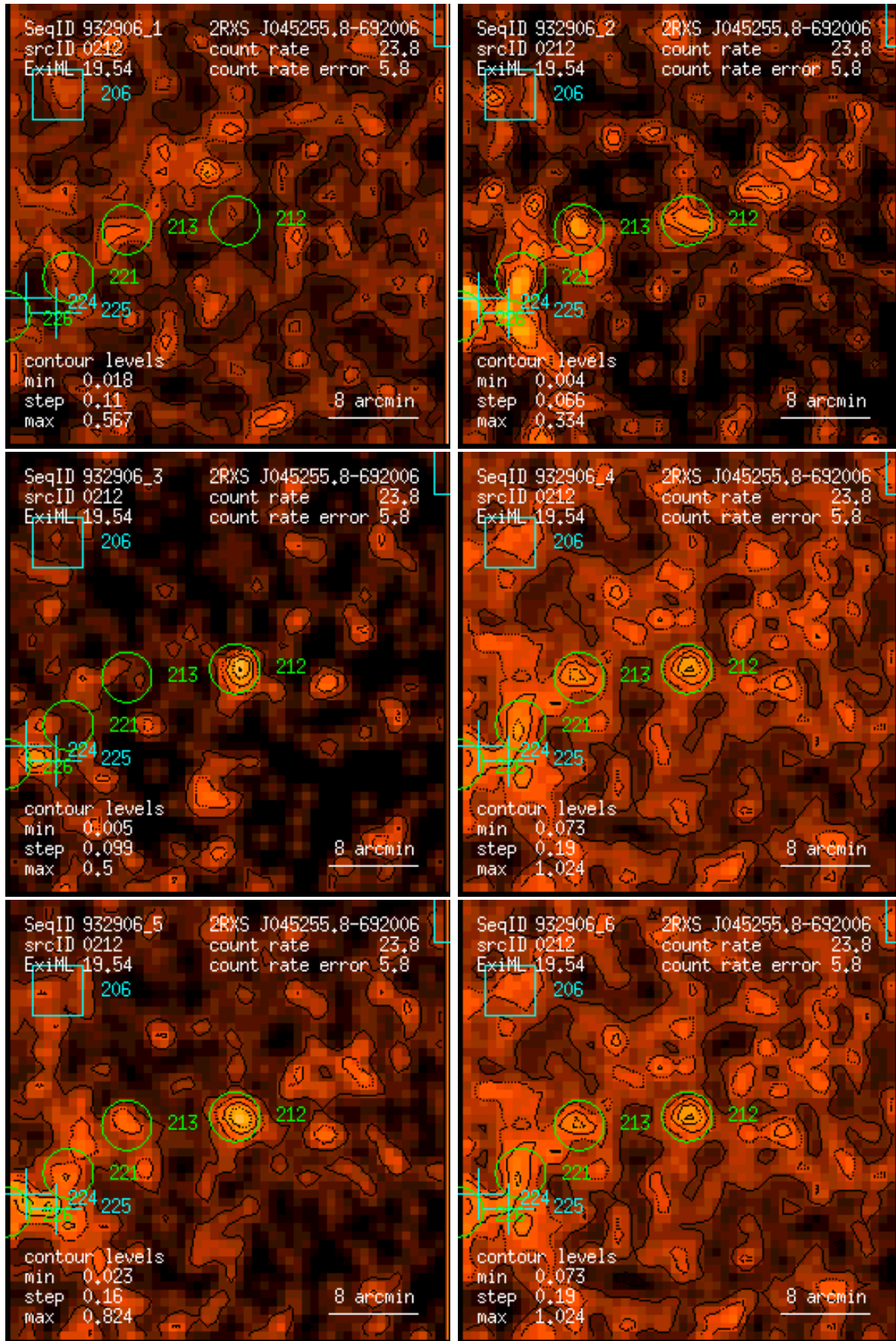
Figure 212: RASS 932906: detection 0212: band rate images, Gaussian filter: (1) PSPC channels 11 – 41, (2) 52 – 90, (3) 91 – 201, (4) 11 – 235, (5) 52 – 201, (6) 11 – 201. Broad band rates in counts/ks. Band rate contour levels in counts/ks/arcmin 2 .
