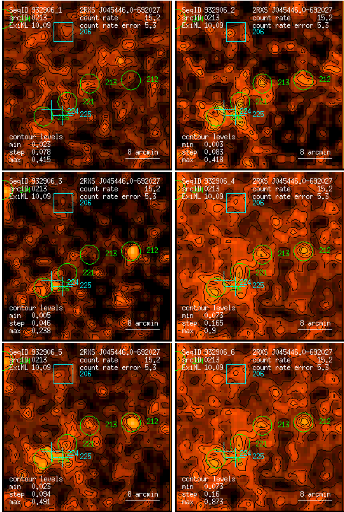
Figure 213: RASS 932906: detection 0213: band rate images, Gaussian filter: (1) PSPC channels 11 – 41, (2) 52 – 90, (3) 91 – 201, (4) 11 – 235, (5) 52 – 201, (6) 11 – 201. Broad band rates in counts/ks. Band rate contour levels in counts/ks/arcmin 2 .
