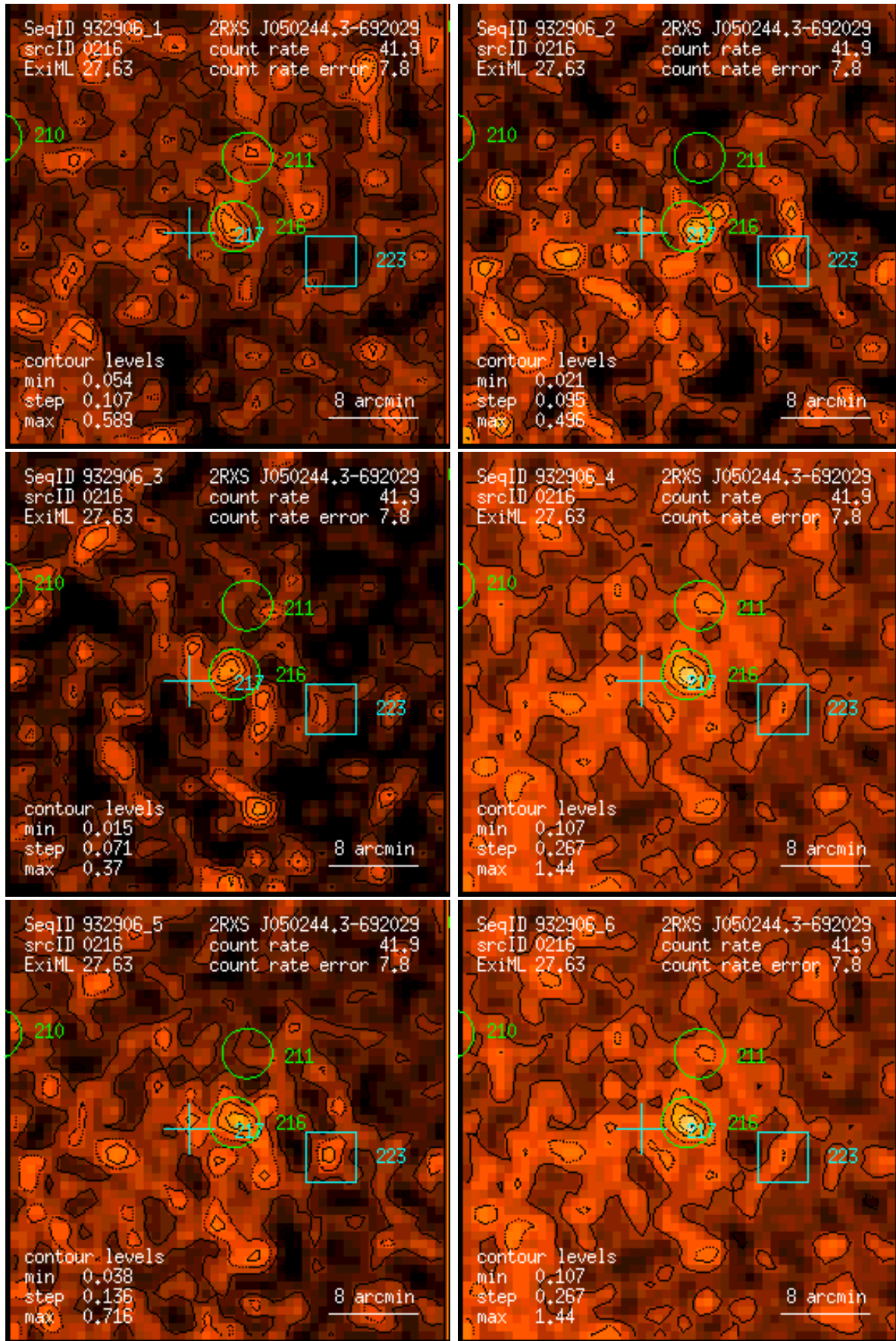
Figure 216: RASS 932906: detection 0216: band rate images, Gaussian filter: (1) PSPC channels 11 – 41, (2) 52 – 90, (3) 91 – 201, (4) 11 – 235, (5) 52 – 201, (6) 11 – 201. Broad band rates in counts/ks. Band rate contour levels in counts/ks/arcmin 2 .
