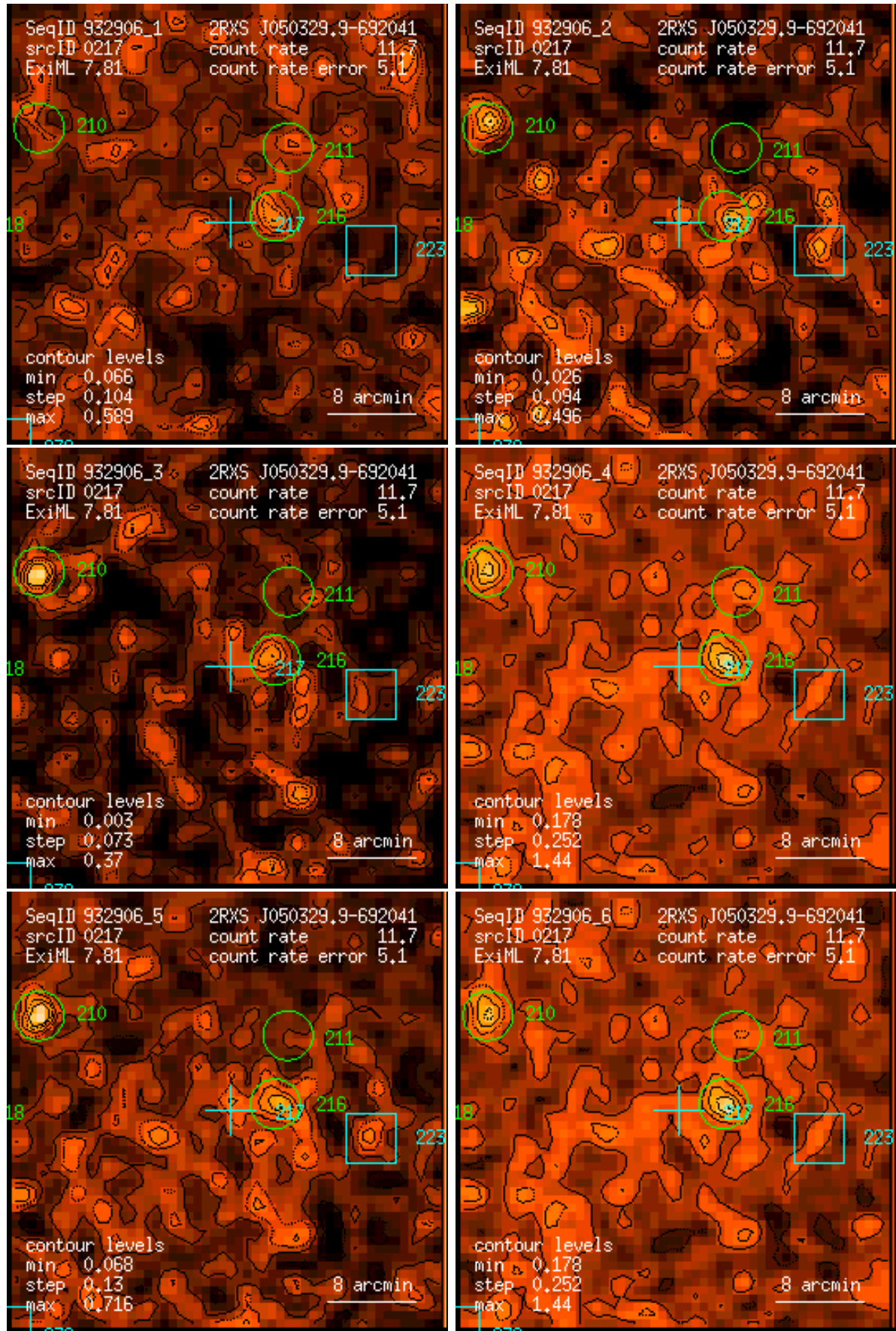
Figure 217: RASS 932906: detection 0217: band rate images, Gaussian filter: (1) PSPC channels 11 – 41, (2) 52 – 90, (3) 91 – 201, (4) 11 – 235, (5) 52 – 201, (6) 11 – 201. Broad band rates in counts/ks. Band rate contour levels in counts/ks/arcmin 2 .
