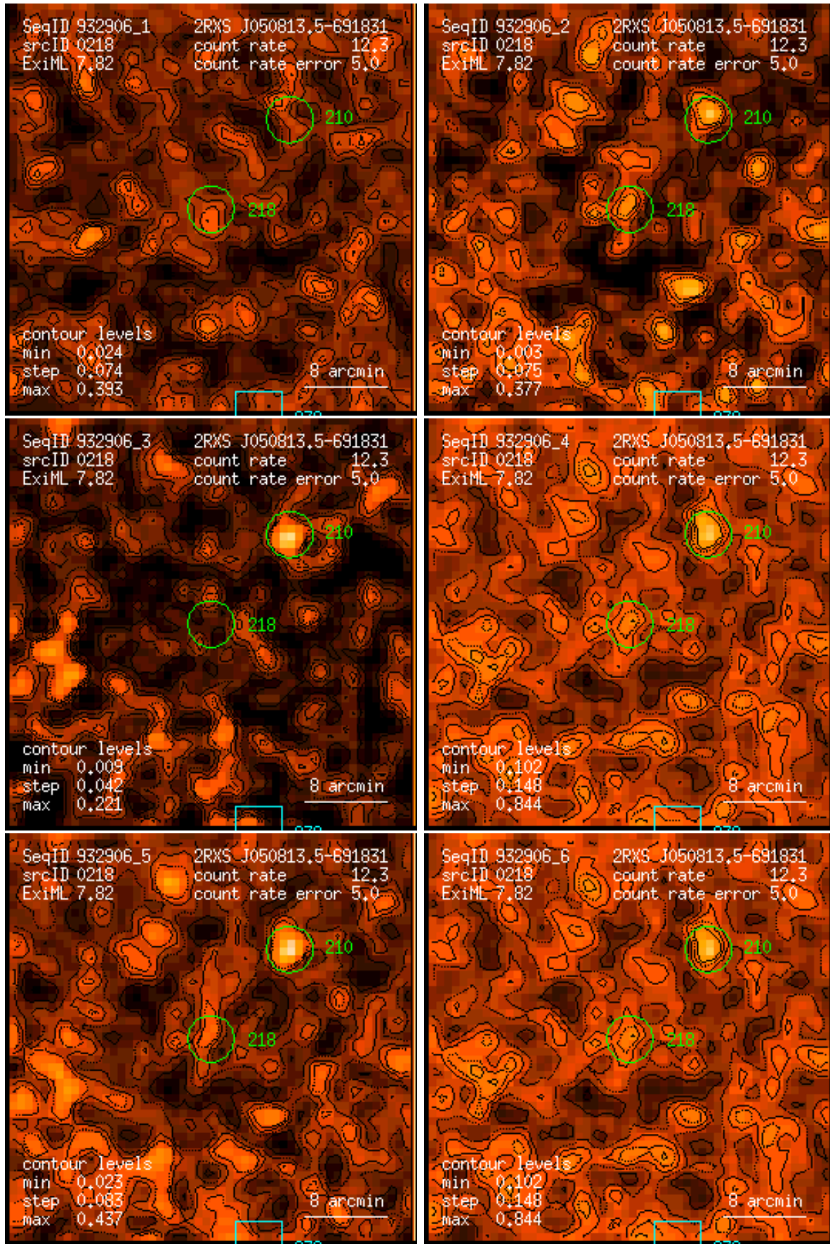
Figure 218: RASS 932906: detection 0218: band rate images, Gaussian filter: (1) PSPC channels 11 – 41, (2) 52 – 90, (3) 91 – 201, (4) 11 – 235, (5) 52 – 201, (6) 11 – 201. Broad band rates in counts/ks. Band rate contour levels in counts/ks/arcmin 2 .
