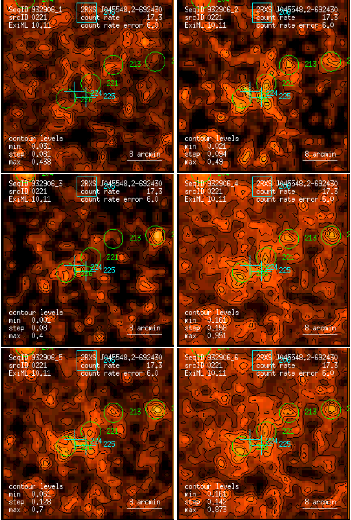
Figure 221: RASS 932906: detection 0221: band rate images, Gaussian filter: (1) PSPC channels 11 – 41, (2) 52 – 90, (3) 91 – 201, (4) 11 – 235, (5) 52 – 201, (6) 11 – 201. Broad band rates in counts/ks. Band rate contour levels in counts/ks/arcmin 2 .
