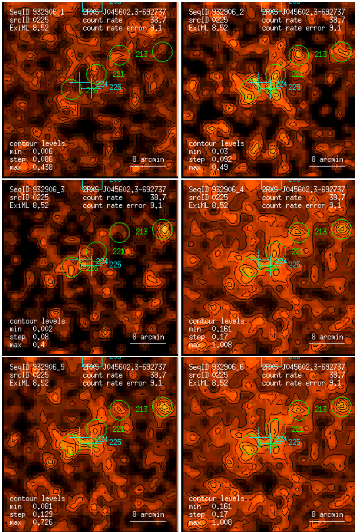
Figure 225: RASS 932906: detection 0225: band rate images, Gaussian filter: (1) PSPC channels 11 – 41, (2) 52 – 90, (3) 91 – 201, (4) 11 – 235, (5) 52 – 201, (6) 11 – 201. Broad band rates in counts/ks. Band rate contour levels in counts/ks/arcmin 2 .
