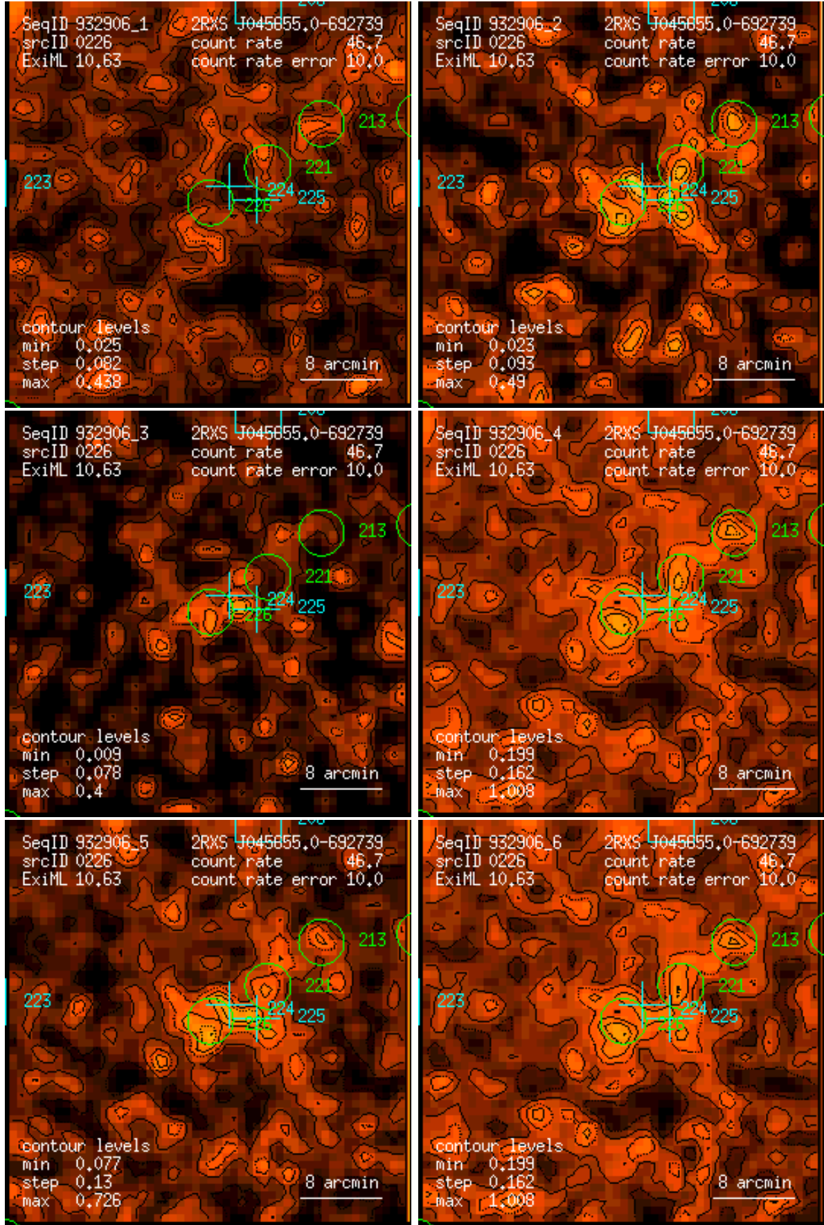
Figure 226: RASS 932906: detection 0226: band rate images, Gaussian filter: (1) PSPC channels 11 – 41, (2) 52 – 90, (3) 91 – 201, (4) 11 – 235, (5) 52 – 201, (6) 11 – 201. Broad band rates in counts/ks. Band rate contour levels in counts/ks/arcmin 2 .
