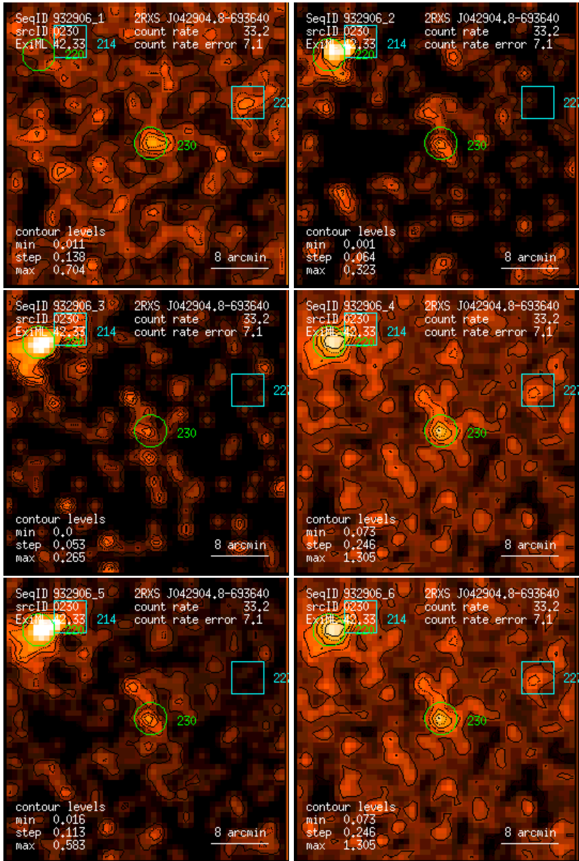
Figure 230: RASS 932906: detection 0230: band rate images, Gaussian filter: (1) PSPC channels 11 – 41, (2) 52 – 90, (3) 91 – 201, (4) 11 – 235, (5) 52 – 201, (6) 11 – 201. Broad band rates in counts/ks. Band rate contour levels in counts/ks/arcmin 2 .
