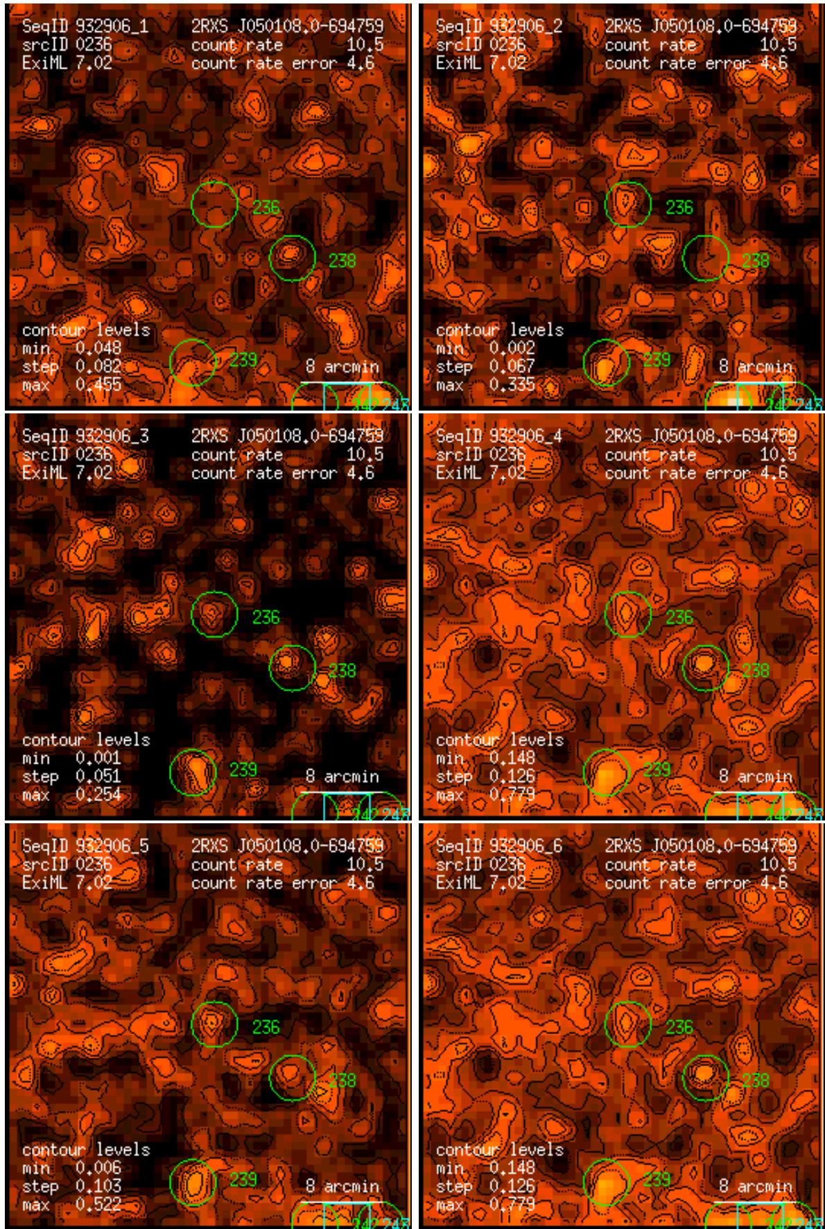
Figure 236: RASS 932906: detection 0236: band rate images, Gaussian filter: (1) PSPC channels 11 – 41, (2) 52 – 90, (3) 91 – 201, (4) 11 – 235, (5) 52 – 201, (6) 11 – 201. Broad band rates in counts/ks. Band rate contour levels in counts/ks/arcmin 2 .
