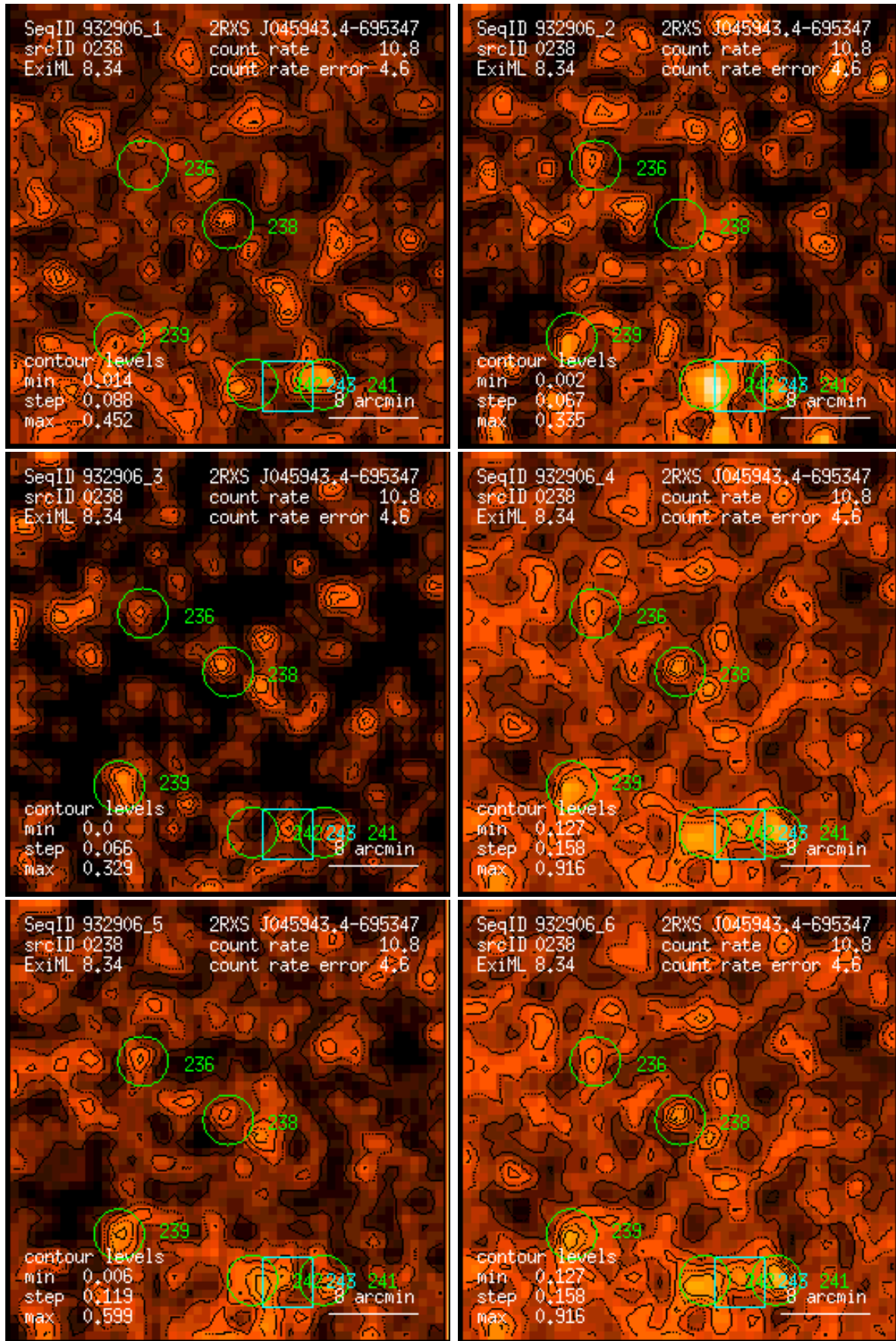
Figure 238: RASS 932906: detection 0238: band rate images, Gaussian filter: (1) PSPC channels 11 – 41, (2) 52 – 90, (3) 91 – 201, (4) 11 – 235, (5) 52 – 201, (6) 11 – 201. Broad band rates in counts/ks. Band rate contour levels in counts/ks/arcmin 2 .
