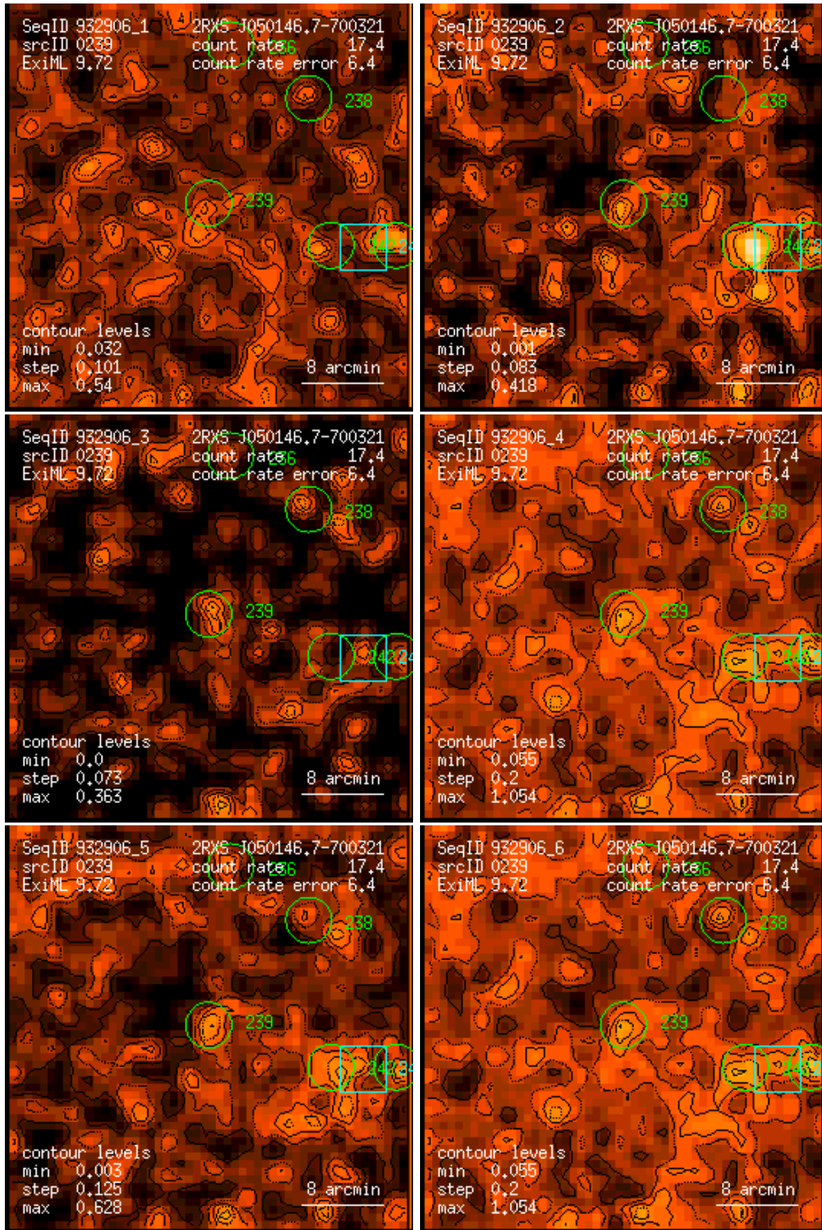
Figure 239: RASS 932906: detection 0239: band rate images, Gaussian filter: (1) PSPC channels 11 – 41, (2) 52 – 90, (3) 91 – 201, (4) 11 – 235, (5) 52 – 201, (6) 11 – 201. Broad band rates in counts/ks. Band rate contour levels in counts/ks/arcmin 2 .
