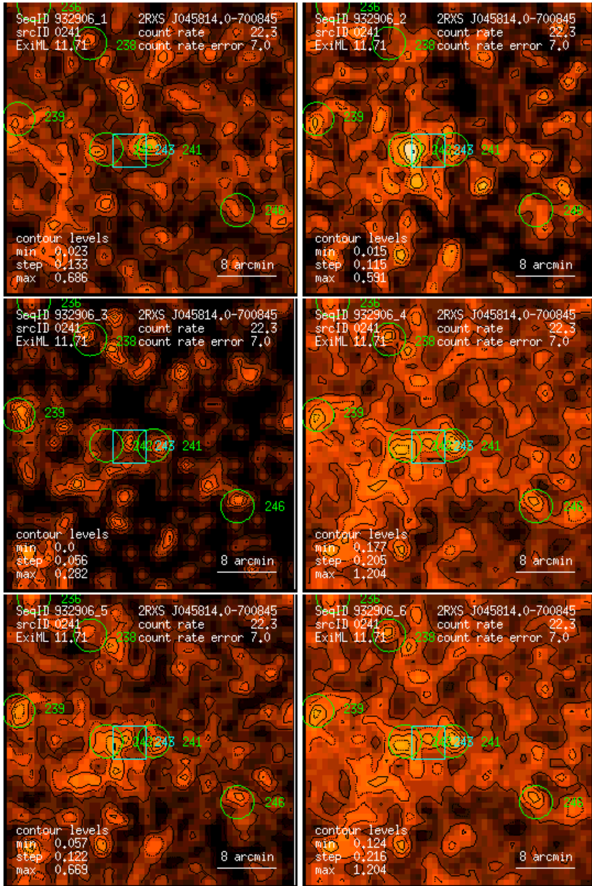
Figure 241: RASS 932906: detection 0241: band rate images, Gaussian filter: (1) PSPC channels 11 – 41, (2) 52 – 90, (3) 91 – 201, (4) 11 – 235, (5) 52 – 201, (6) 11 – 201. Broad band rates in counts/ks. Band rate contour levels in counts/ks/arcmin 2 .
