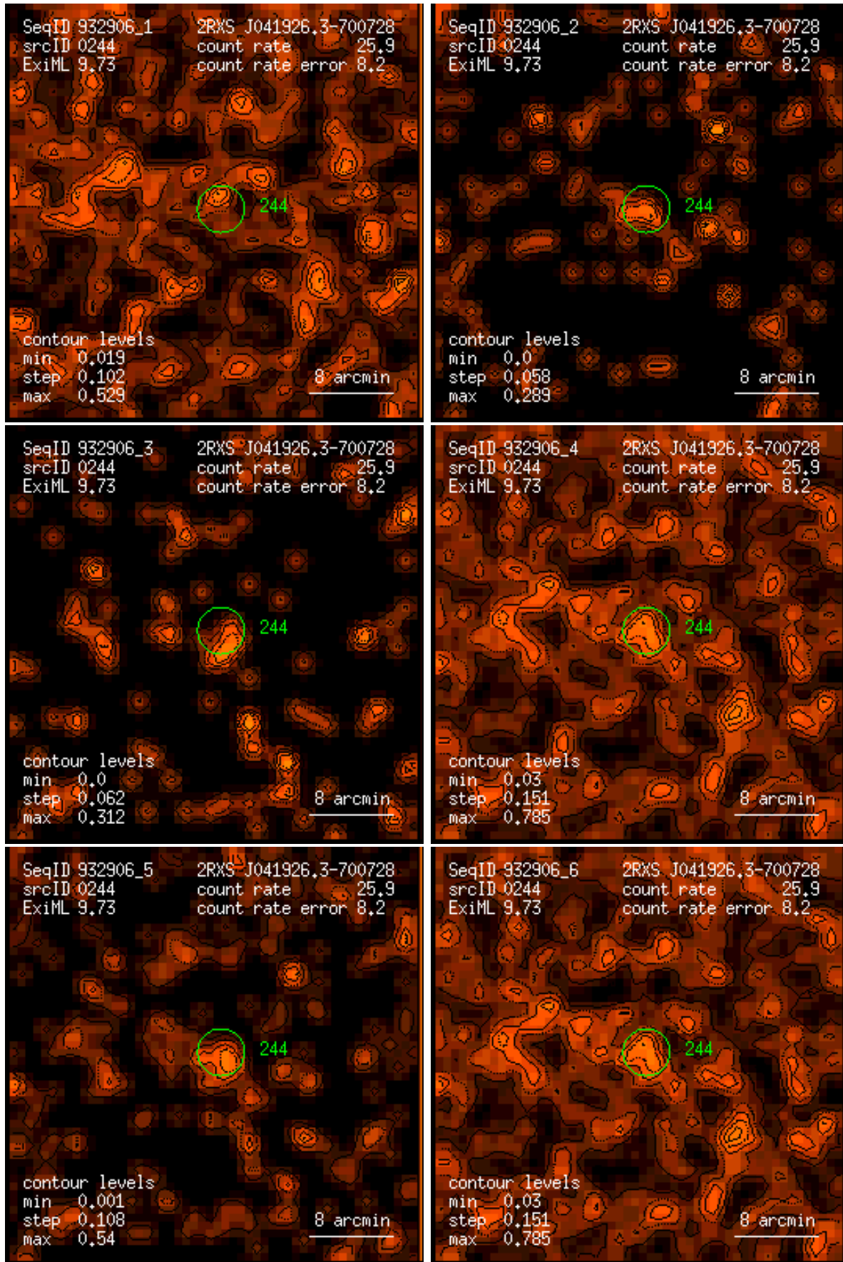
Figure 244: RASS 932906: detection 0244: band rate images, Gaussian filter: (1) PSPC channels 11 – 41, (2) 52 – 90, (3) 91 – 201, (4) 11 – 235, (5) 52 – 201, (6) 11 – 201. Broad band rates in counts/ks. Band rate contour levels in counts/ks/arcmin 2 .
